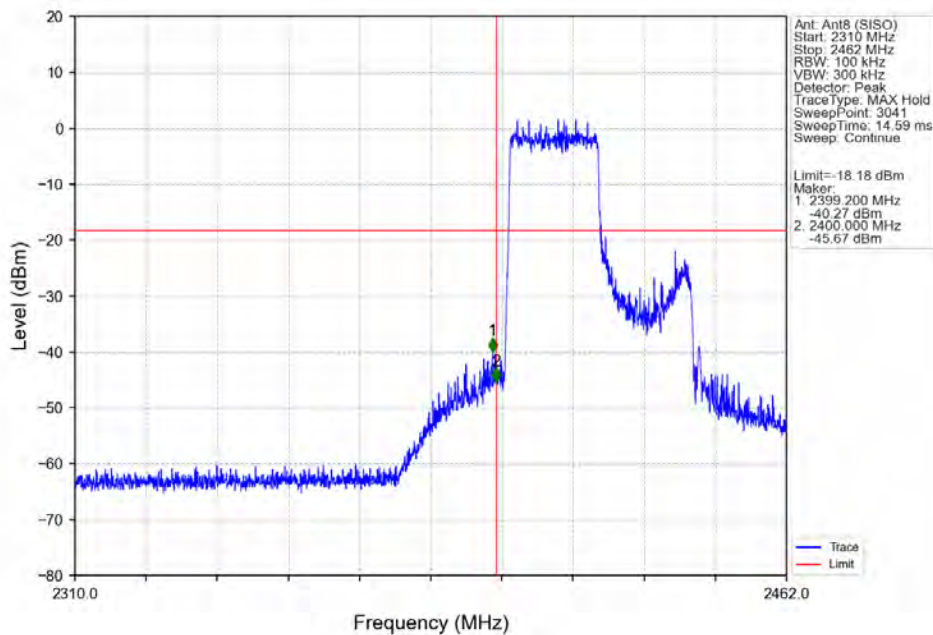
802.11ax(HEW40)_LCH_2422MHz_RU242_Left_Ant8 (SISO)_NTNV
