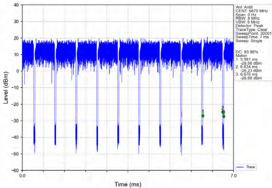
802.11ac(VHT40)_HCH_5670MHz_Ant8_NTNV
