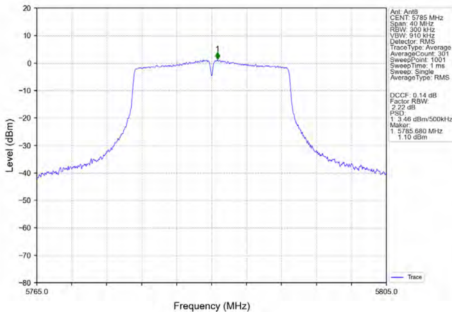
802.11ac(VHT20)_MCH_5785MHz_Ant8_NTNV
