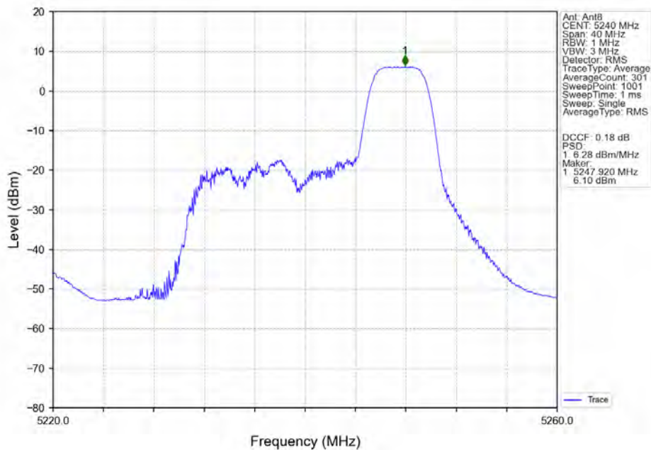
802.11ax(HEW20)_HCH_5240MHz_RU52_Right_Ant8_NTNV
