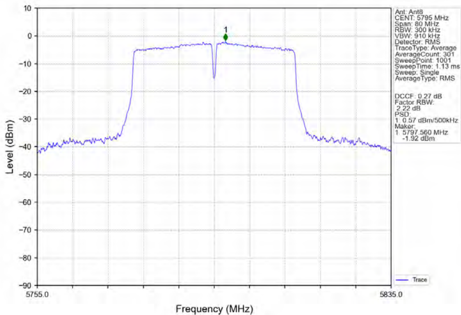
802.11n(HT40)_HCH_5795MHz_Ant8_NTNV
