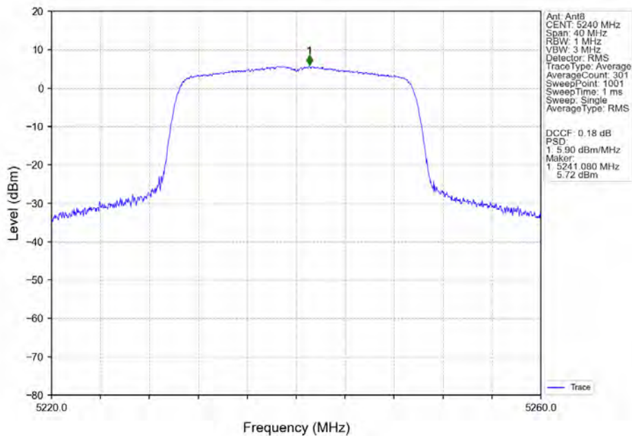
802.11ax(HEW20)_HCH_5240MHz_RU242_Left_Ant8_NTNV
