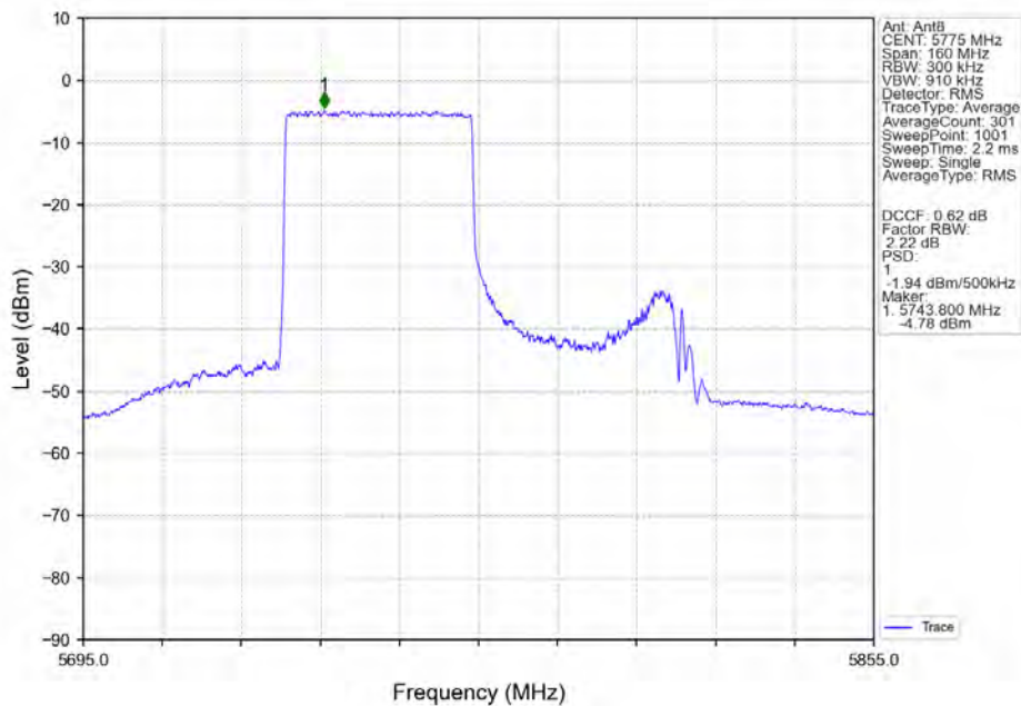
802.11ax(HEW80)_MCH_5775MHz_RU484_Left_Ant8_NTNV
