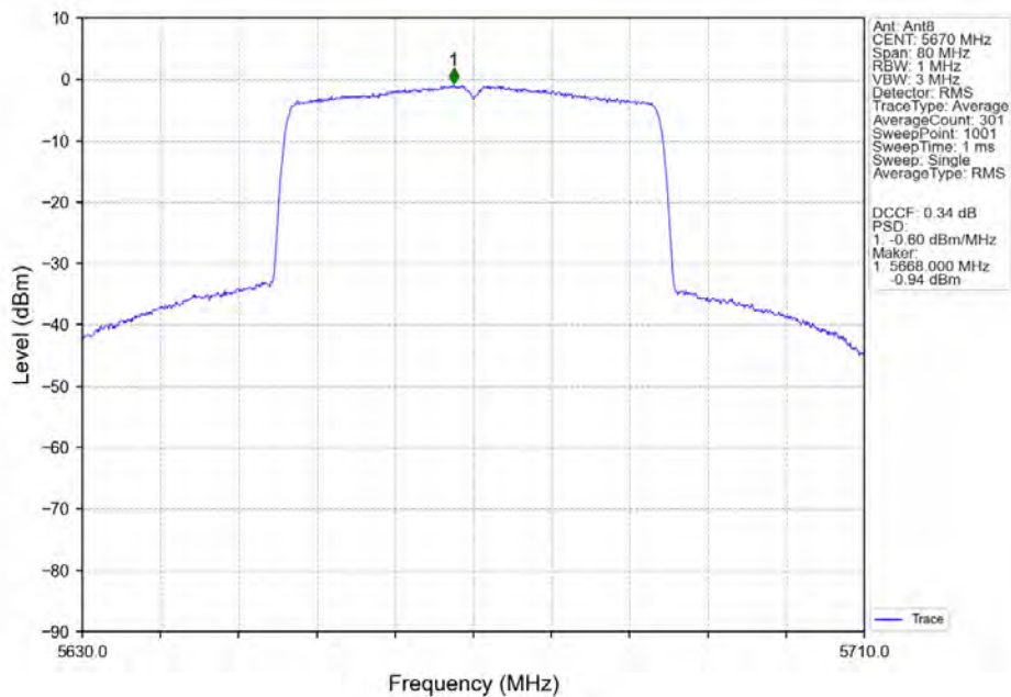
802.11ax(HEW40)_HCH_5670MHz_RU484_Left_Ant8_NTNV
