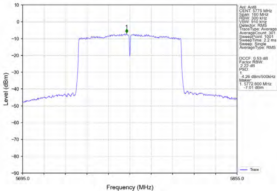
802.11ac(VHT80)_MCH_5775MHz_Ant8_NTNV
