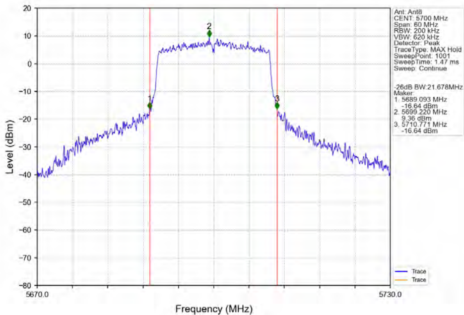
802.11ax(HEW20)_HCH_5700MHz_RU242_Left_Ant8_NTNV
