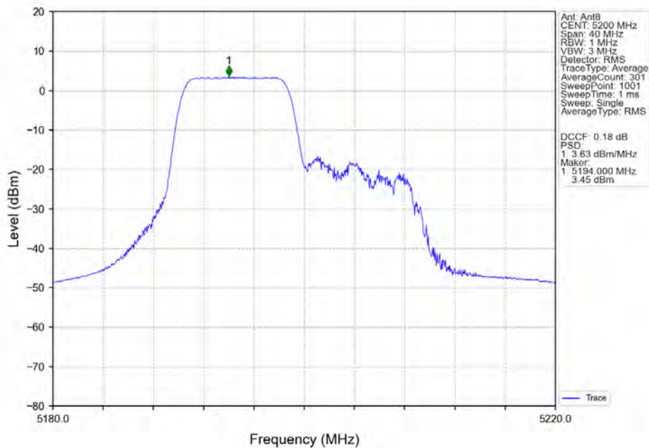
802.11ax(HEW20)_MCH_5200MHz_RU106_Left_Ant8_NTNV
