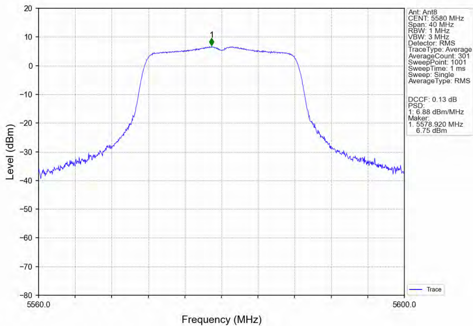
802.11a_MCH_5580MHz_Ant8_NTNV
