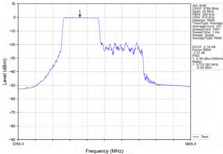
802.11ax(HEW20)_MCH_5785MHz_RU242_Left_Ant8_NTNV
