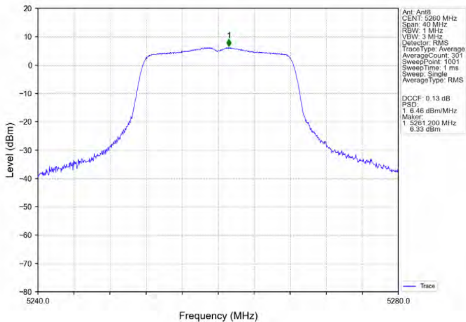
802.11a_LCH_5260MHz_Ant8_NTNV
