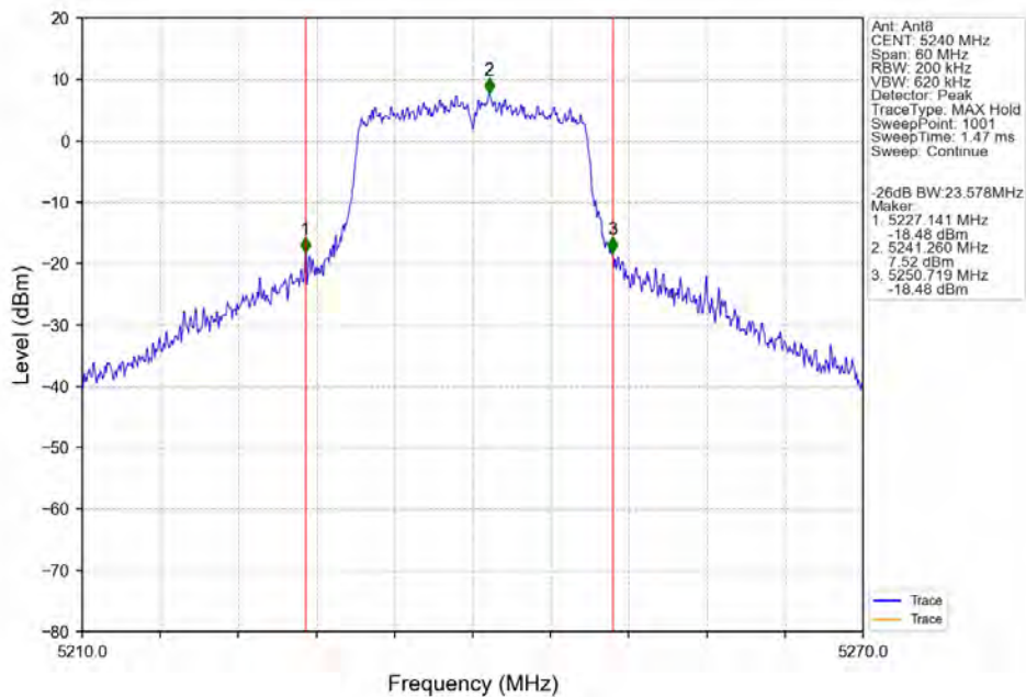
802.11ac(VHT20)_HCH_5240MHz_Ant8_NTNV
