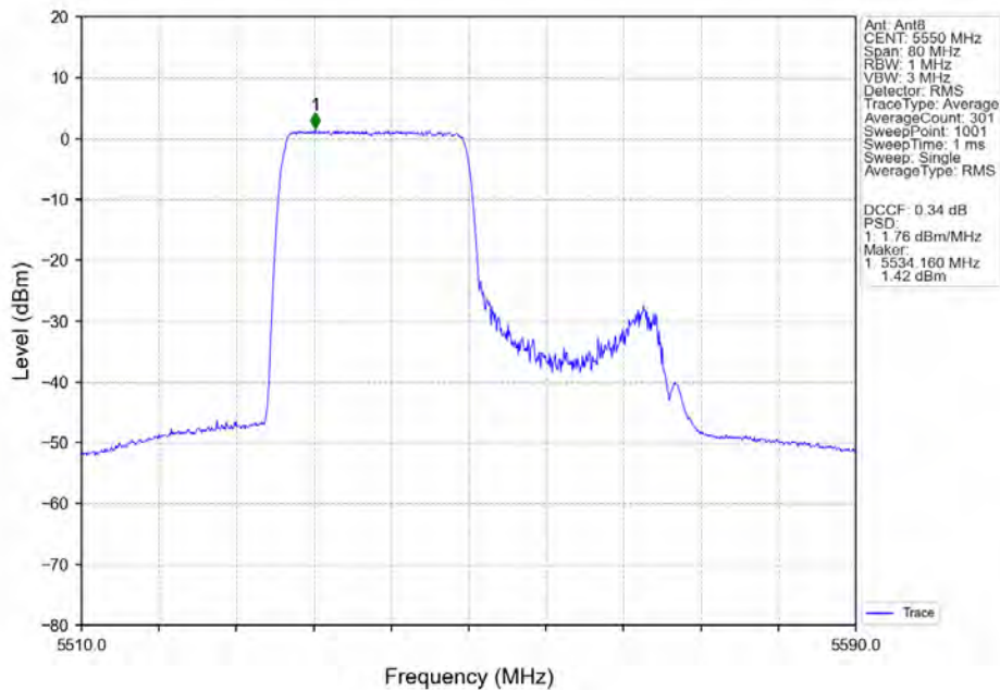
802.11ax(HEW40)_MCH_5550MHz_RU484_Left_Ant8_NTNV
