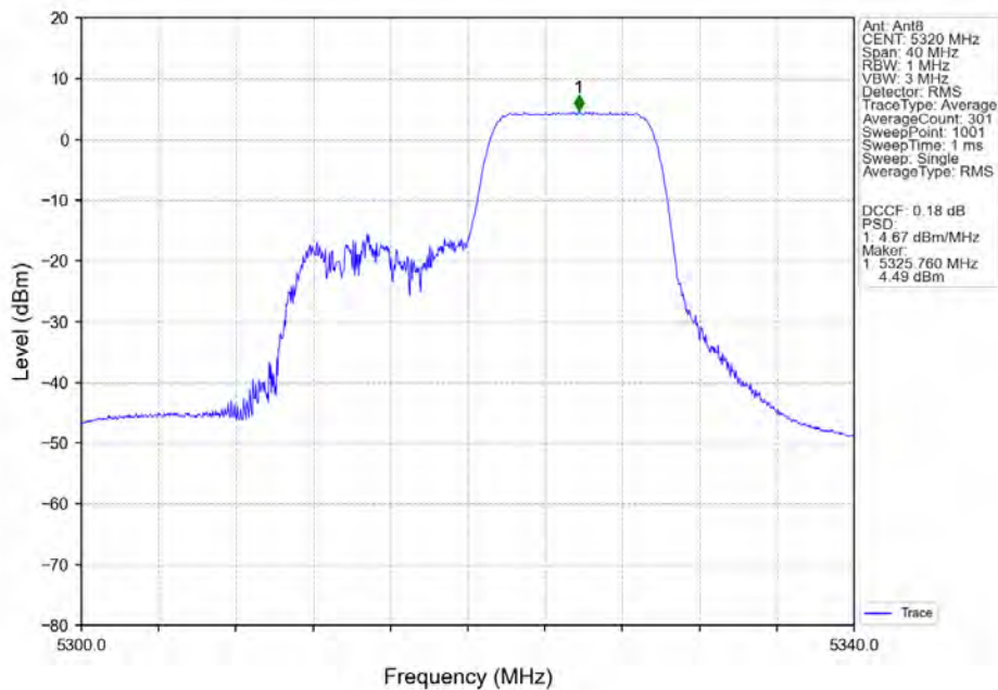
802.11ax(HEW20)_HCH_5320MHz_RU106_Right_Ant8_NTNV
