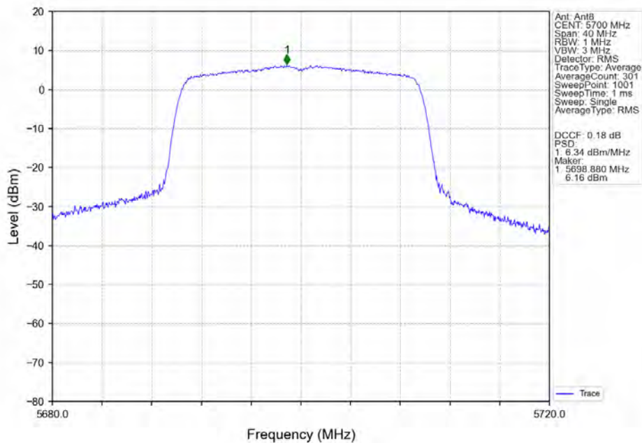
802.11ax(HEW20)_HCH_5700MHz_RU242_Left_Ant8_NTNV
