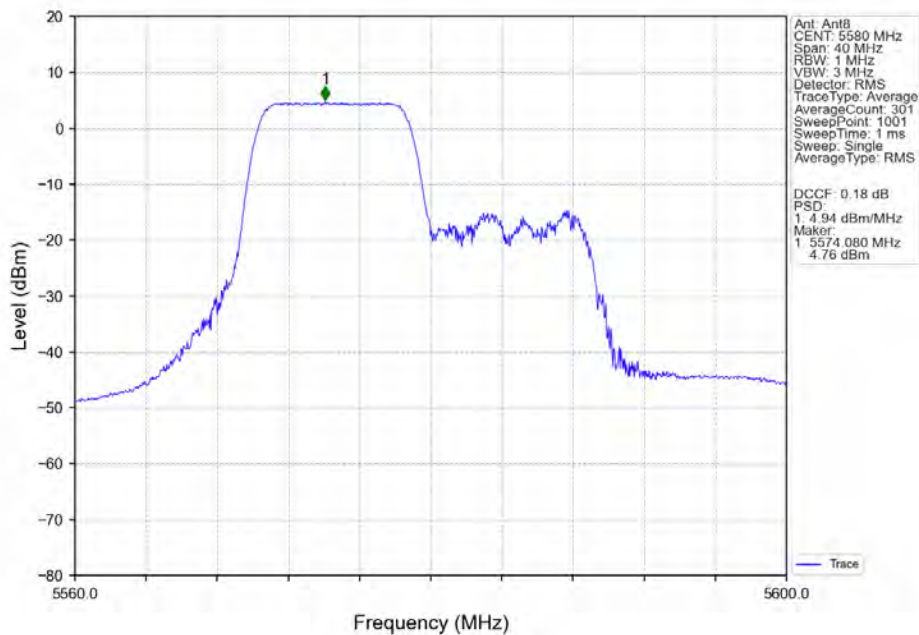
802.11ax(HEW20)_MCH_5580MHz_RU106_Left_Ant8_NTNV
