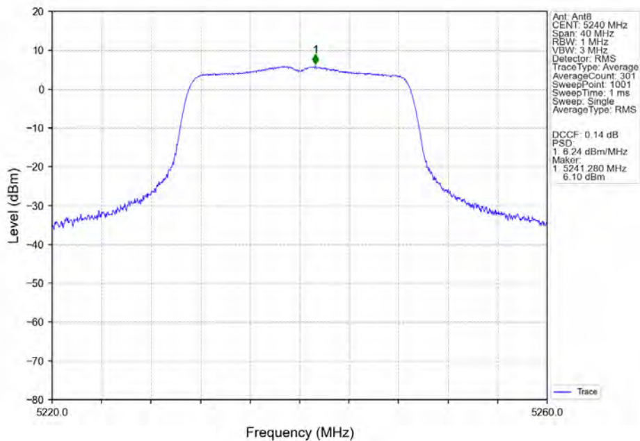
802.11ac(VHT20)_HCH_5240MHz_Ant8_NTNV
