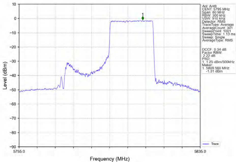
802.11ax(HEW40)_HCH_5795MHz_RU242_Right_Ant8_NTNV
