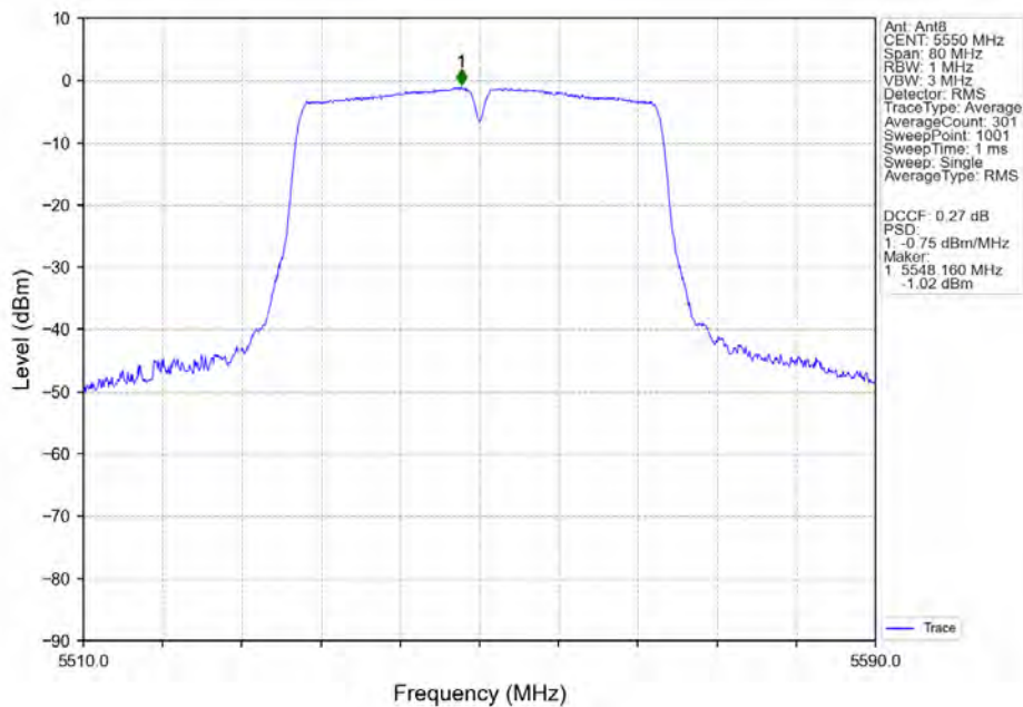
802.11n(HT40)_MCH_5550MHz_Ant8_NTNV
