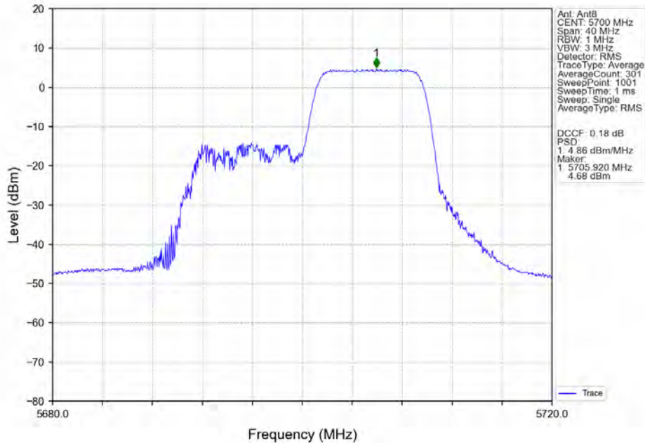
802.11ax(HEW20)_HCH_5700MHz_RU242_Left_Ant8_NTNV
