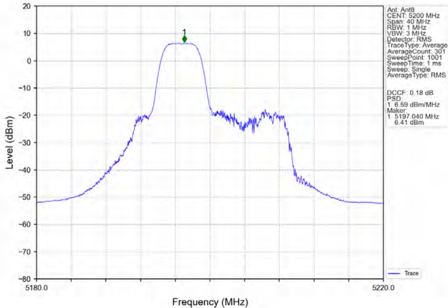
802.11ax(HEW20)_MCH_5200MHz_RU106_Left_Ant8_NTNV
