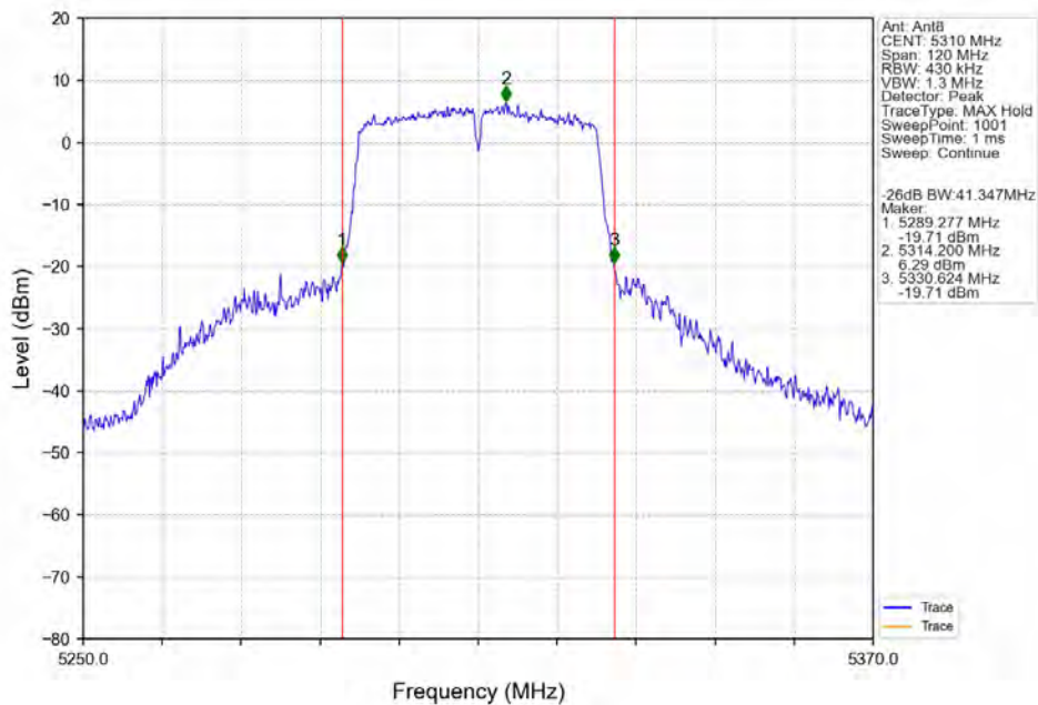
802.11ac(VHT40)_HCH_5310MHz_Ant8_NTNV
