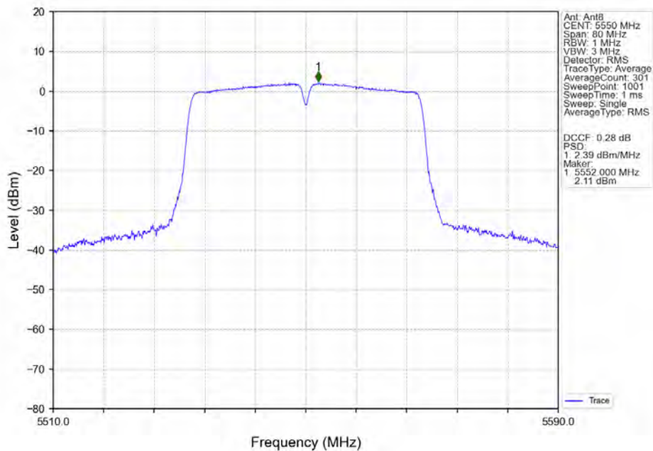
802.11ac(VHT40)_MCH_5550MHz_Ant8_NTNV
