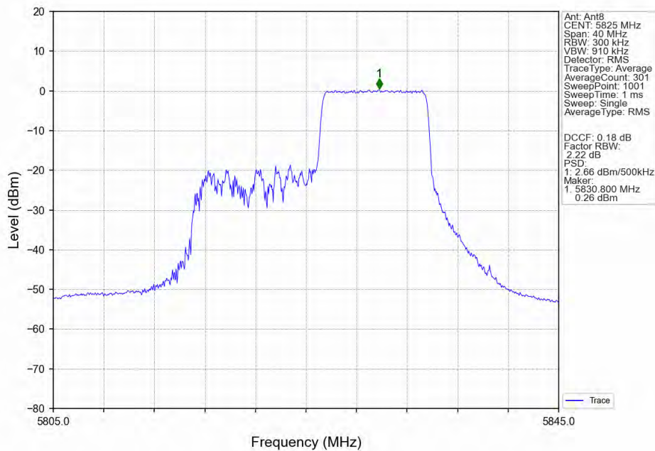
802.11ax(HEW20)_HCH_5825MHz_RU106_Right_Ant8_NTNV
