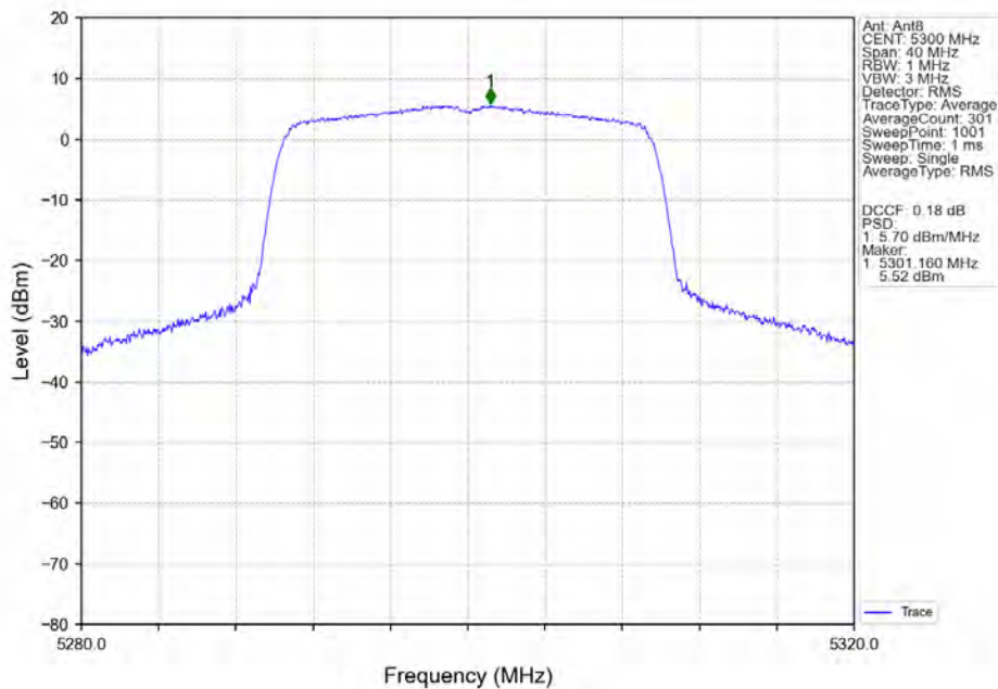
802.11ax(HEW20)_MCH_5300MHz_RU242_Left_Ant8_NTNV
