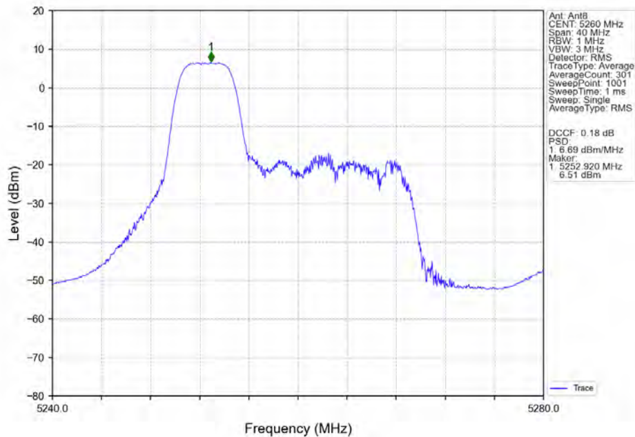
802.11ax(HEW20)_LCH_5260MHz_RU106_Left_Ant8_NTNV
