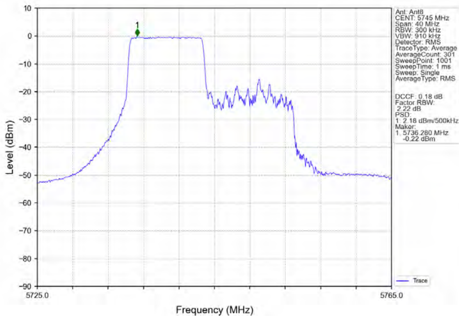
802.11ax(HEW20)_LCH_5745MHz_RU106_Left_Ant8_NTNV
