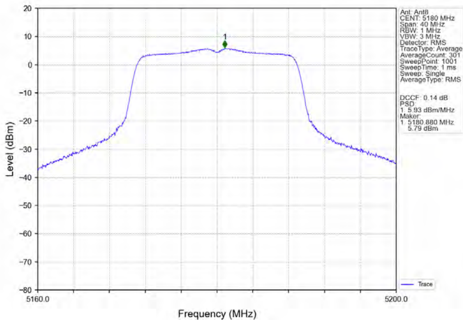
802.11ac(VHT20)_LCH_5180MHz_Ant8_NTNV
