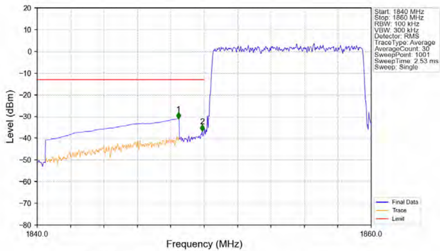
Band2_10MHz_64QAM_LCH_1855MHz_RB_50_0_NTN
