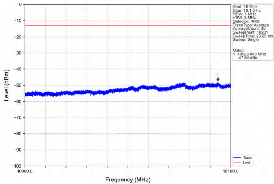
Band2_10MHz_64QAM_LCH_1855MHz_RB_50_0_NTN
