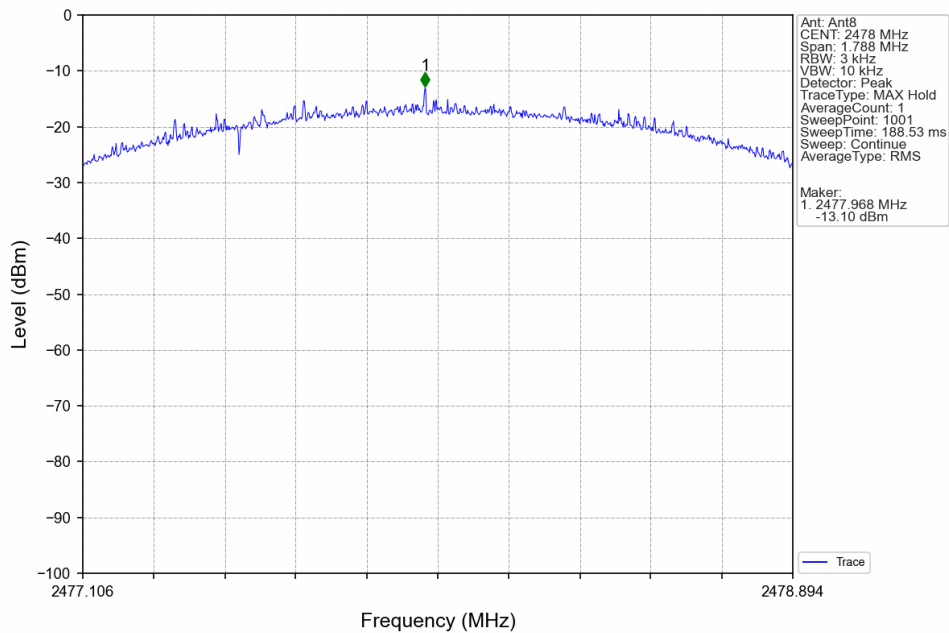
2M_HCH_2478MHz_Ant8_NTNV
