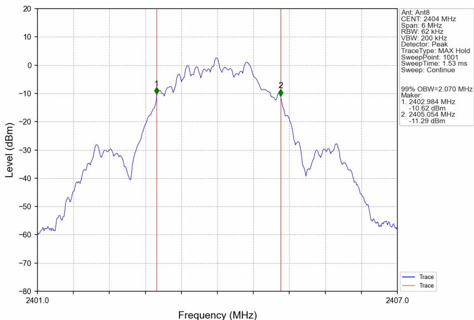
2M_LCH_2404MHz_Ant8_NTNV
