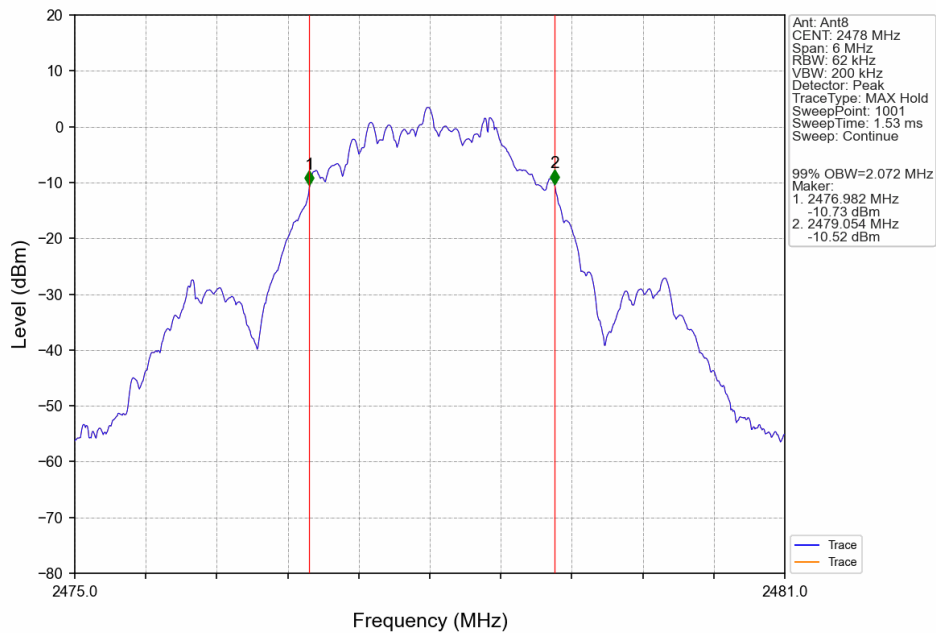
2M_HCH_2478MHz_Ant8_NTNV
