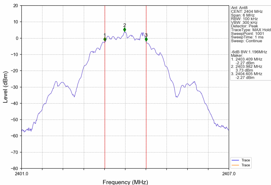
2M_LCH_2404MHz_Ant8_NTNV
