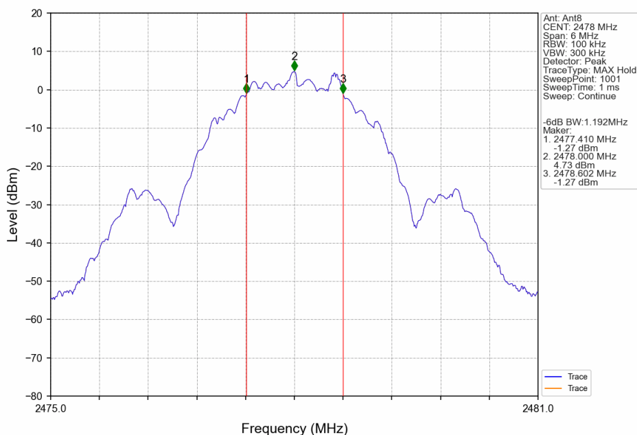
2M_HCH_2478MHz_Ant8_NTNV
