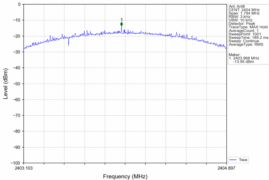
2M_LCH_2404MHz_Ant8_NTNV
