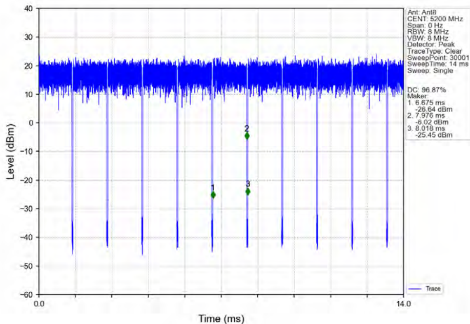
802.11n(HT20)_MCH_5200MHz_Ant8_NTNV
