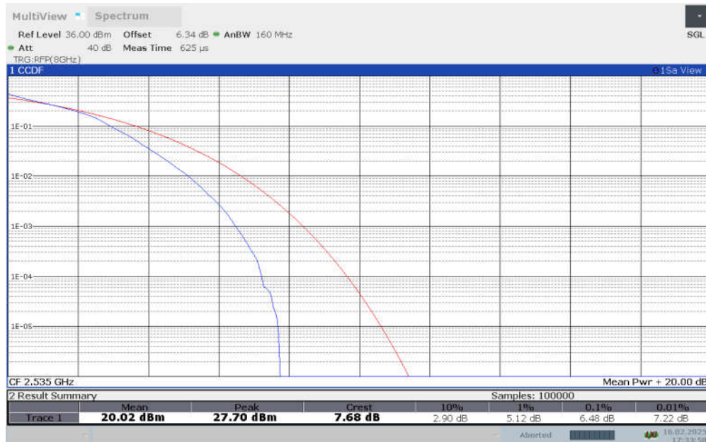
n7, DFT-s-64QAM (PAPR)
