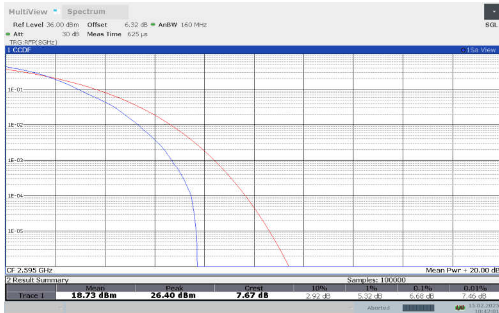
n38, DFT-s-pi/2 BPSK (PAPR)
