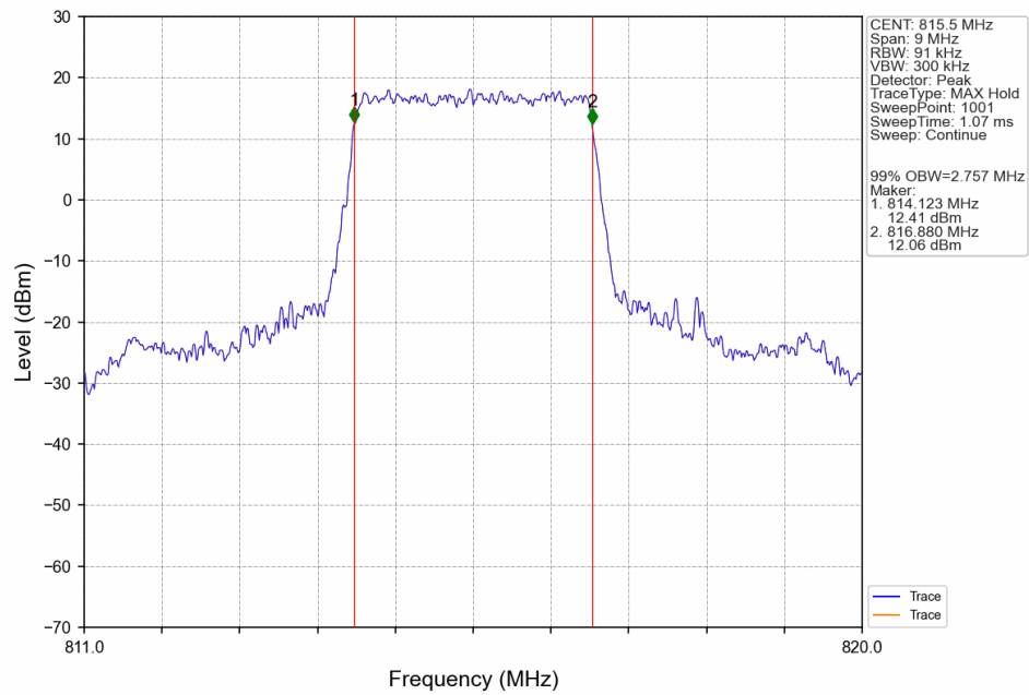
Band26a_3MHz_QPSK_LCH_815.5MHz_RB_15_0_NTNV
