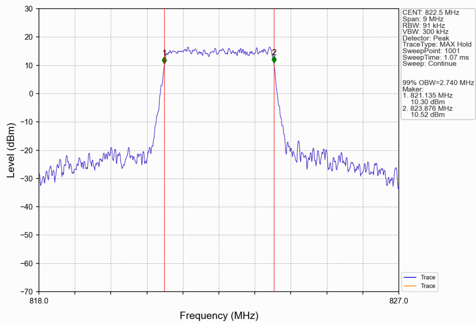
Band26a_3MHz_64QAM_HCH_822.5MHz_RB_15_0_NTNV
