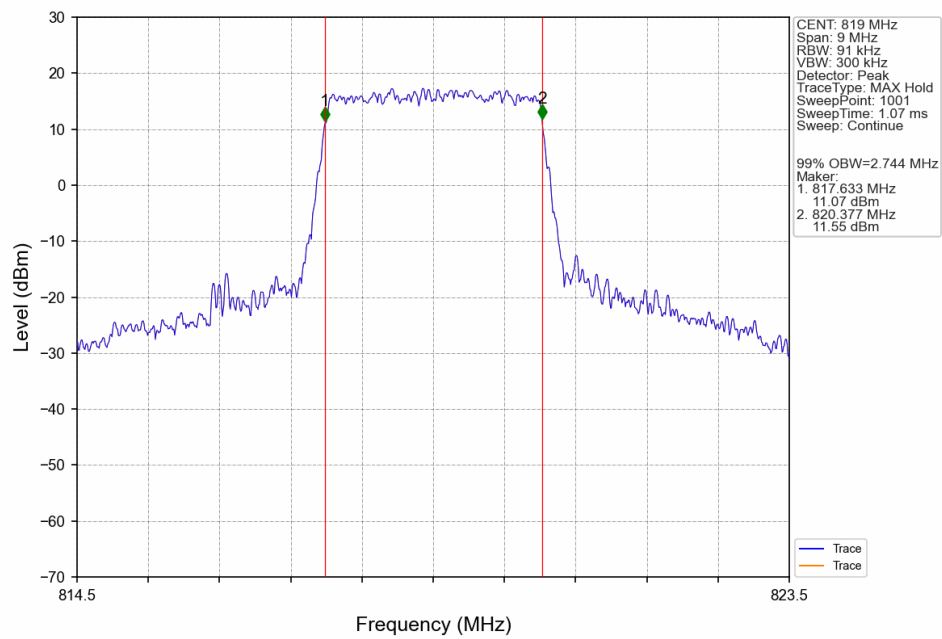
Band26a_3MHz_16QAM_MCH_819MHz_RB_15_0_NTNV
