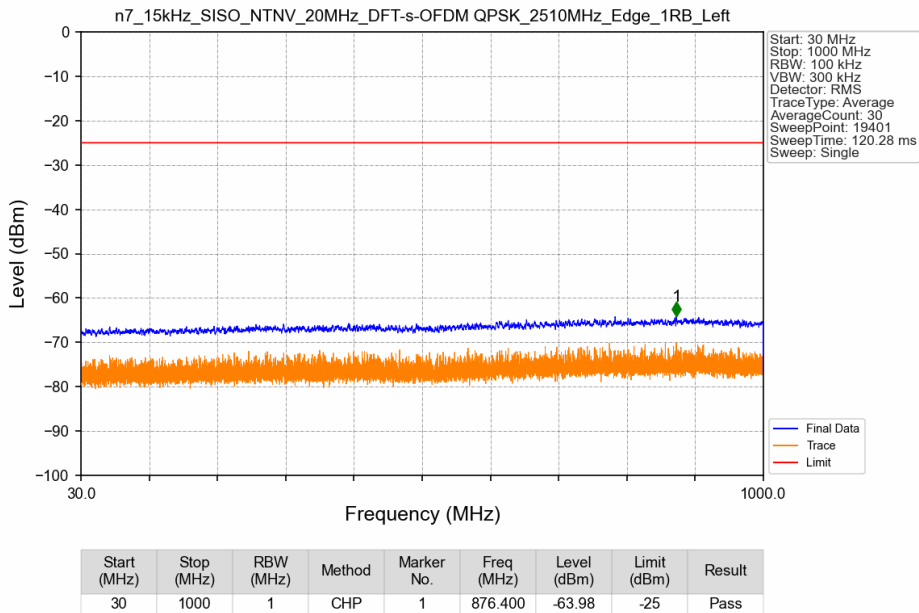
n7_15kHz_SISO_NTNV_20MHz_DFT-s-OFDM QPSK_2510MHz_Edge_1RB_Left_Ant3
