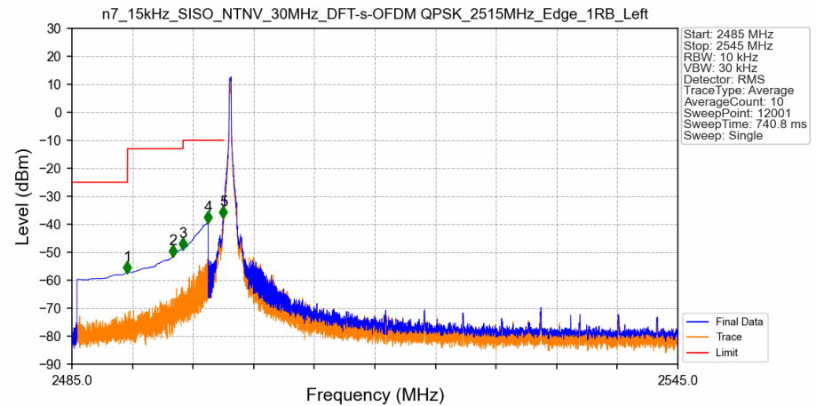
n7_15kHz_SISO_NTNV_30MHz_DFT-s-OFDM QPSK_2515MHz_Edge_1RB_Left_Ant3
