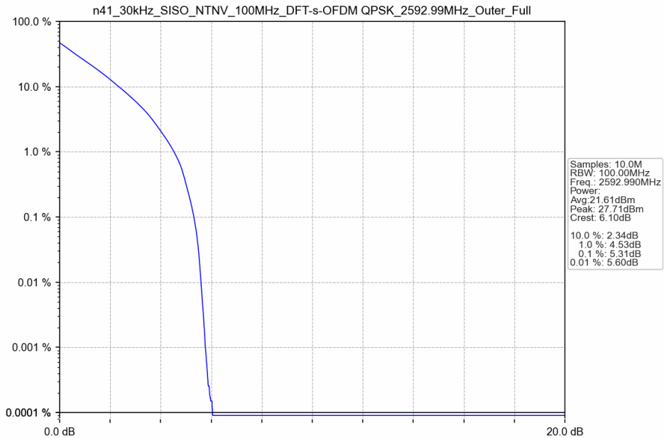
n41_30kHz_SISO_NTNV_100MHz_DFT-s-OFDM QPSK_2592.99MHz_Outer_Full_Ant3
