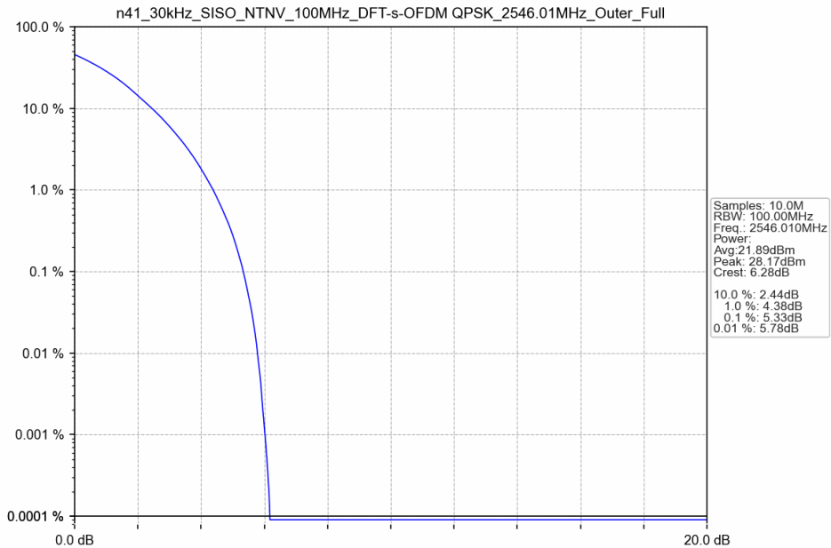
n41_30kHz_SISO_NTNV_100MHz_DFT-s-OFDM QPSK_2546.01MHz_Outer_Full_Ant3
