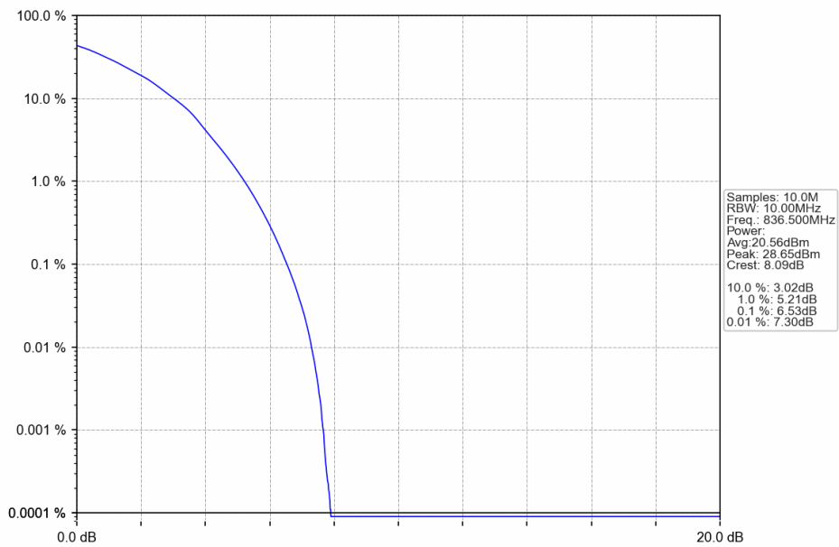
Band5 10MHz 64QAM MCH 836.5MHz RB 50 0 NTN
