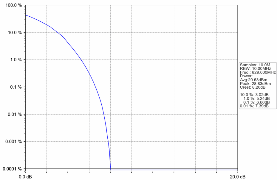
Band5 10MHz 64QAM LCH 829MHz RB 50 0 NTN
