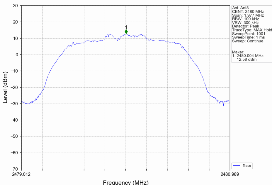
Pi/4DQPSK_2DH5_HCH_2480MHz_Ant8_NTNV
