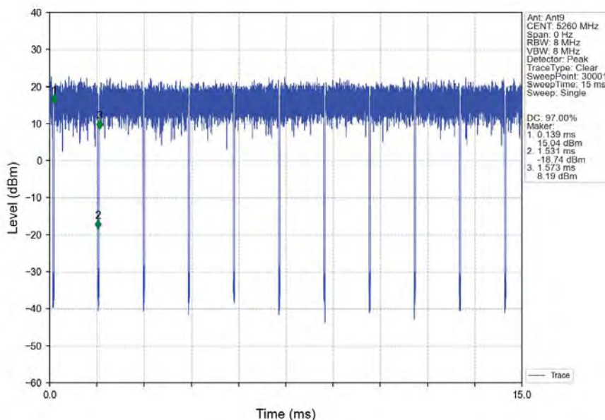
802.11a_LCH_5260MHz_Ant9_NTNV
