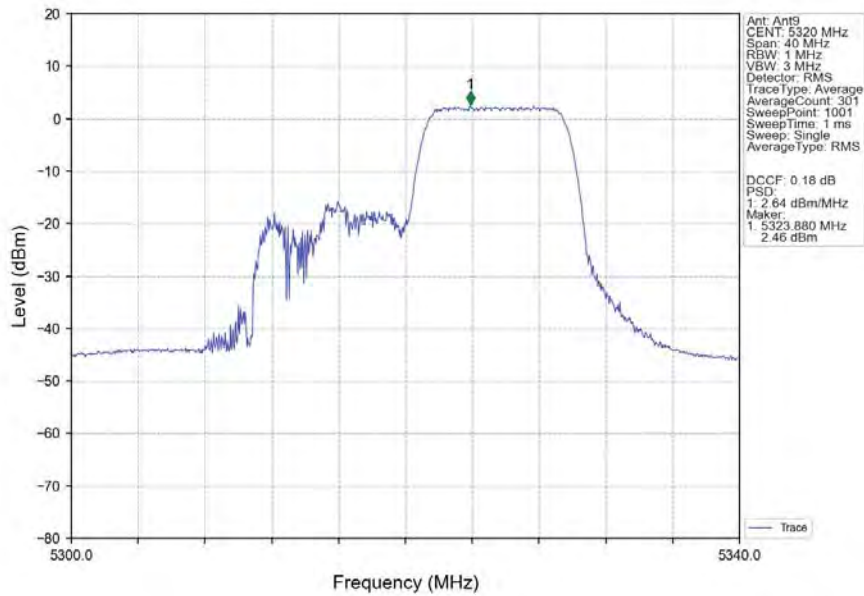
802.11ax(HEW20)_HCH_5320MHz_RU106_Right_Ant9_NTNV
