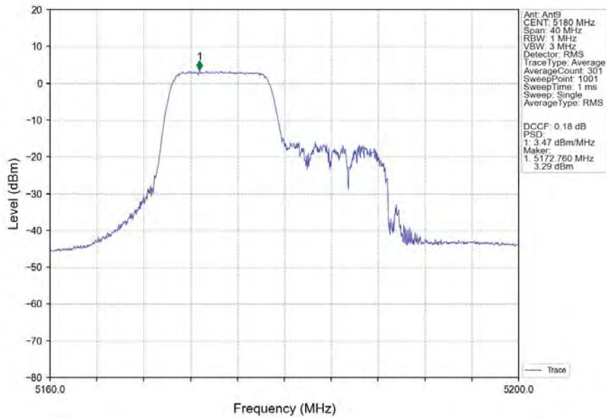
802.11ax(HEW20)_LCH_5180MHz_RU106_Left_Ant9_NTNV
