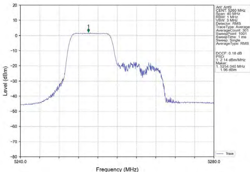
802.11ax(HEW20)_LCH_5260MHz_RU106_Left_Ant9_NTNV
