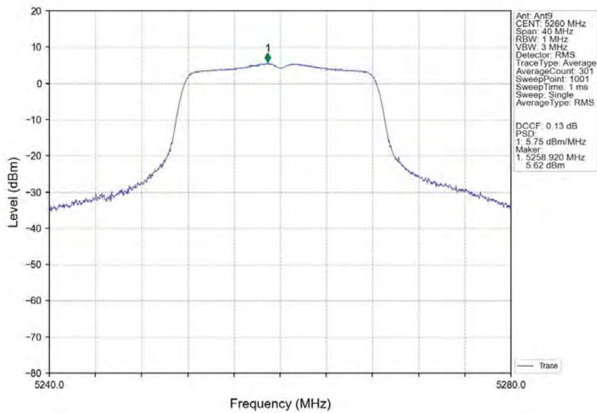
802.11a_LCH_5260MHz_Ant9_NTNV
