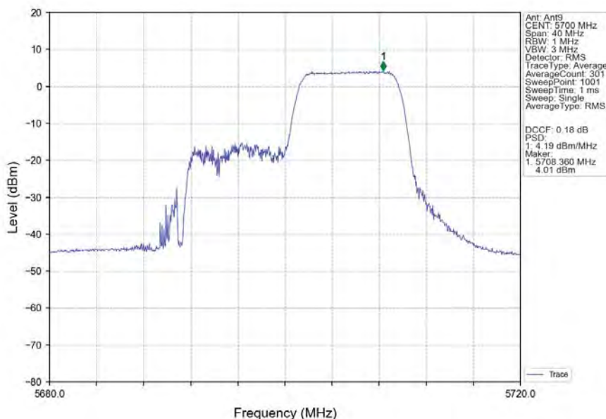
802.11ax(HEW20)_HCH_5700MHz_RU106_Right_Ant9_NTNV
