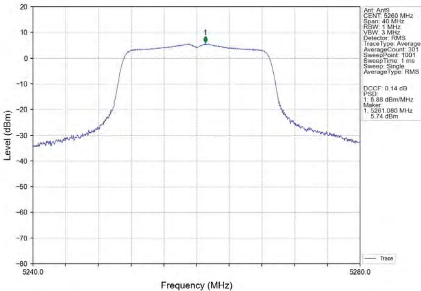
802.11ac(VHT20)_LCH_5260MHz_Ant9_NTNV
