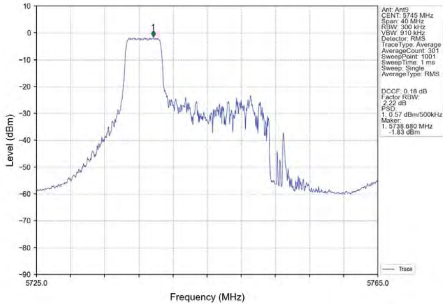
802.11ax(HEW20)_LCH_5745MHz_RU52_Left_Ant9_NTNV
