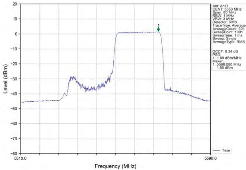
802.11ax(HEW40)_MCH_5550MHz_RU242_Right_Ant9_NTNV
