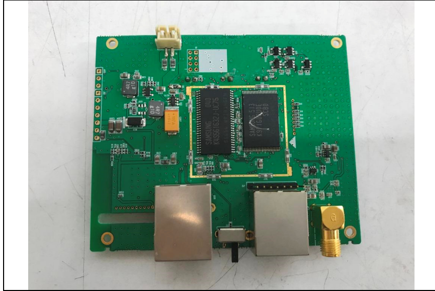
Top view of Main PCB
