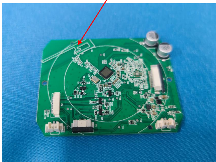
PCB Antenna
