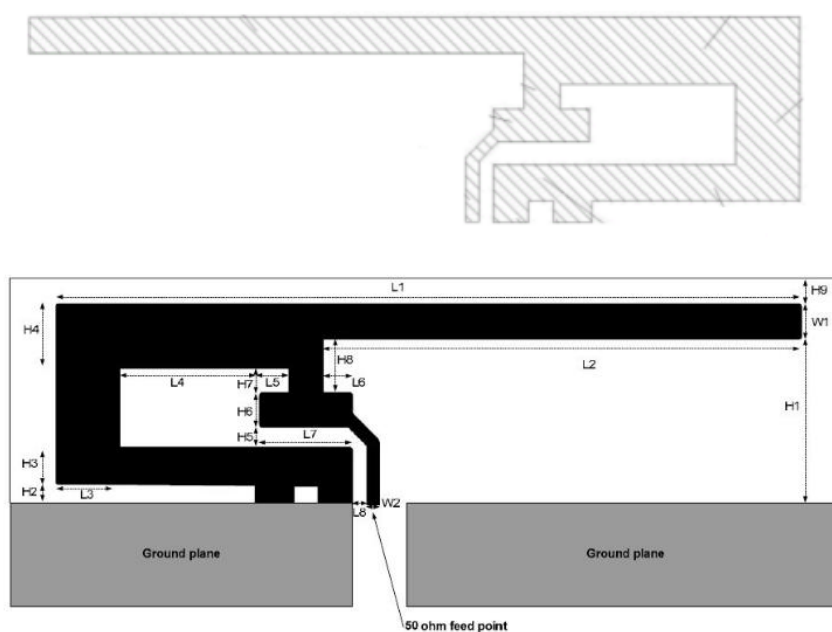
Figure 1. IFA Dimensions
