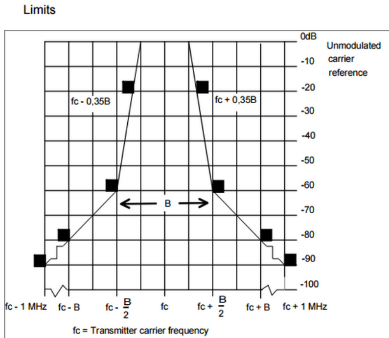
Figure 3: Spectrum mask for analogue systems in all bands
