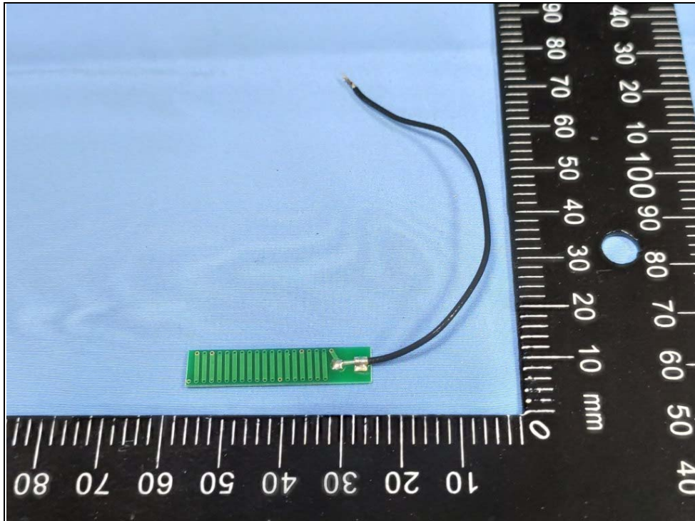
RF Antenna
