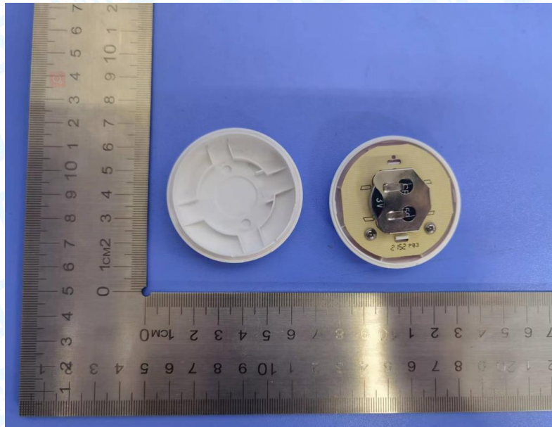
Photo 7 Appearance of PCB
