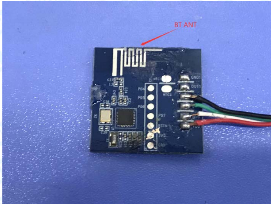
Model: XHBT01 Photo 2 Internal of EUT
