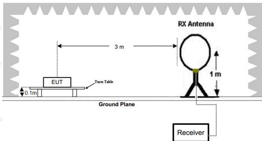
(A) Radiated Emission Test Set-Up, Frequency Below 30MHz.
