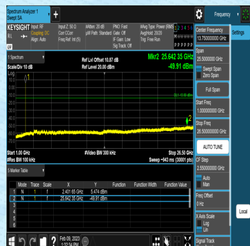
2DH5-Ant1-2402-1000~26500-6.20
