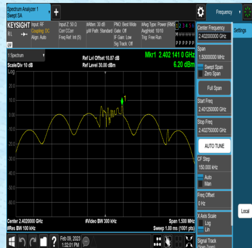
2DH5-Ant1-2402-Reference-6.20
