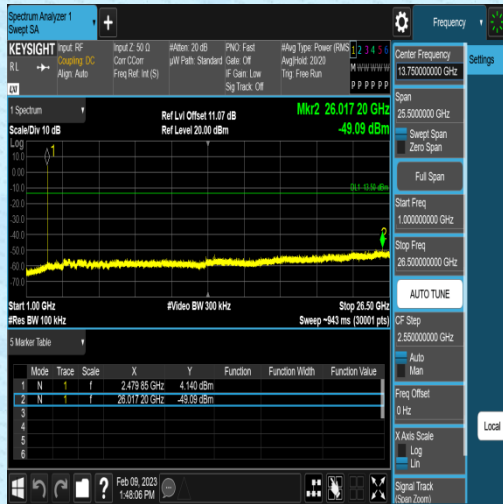
3DH5-Ant1-2480-1000~26500-6.50
