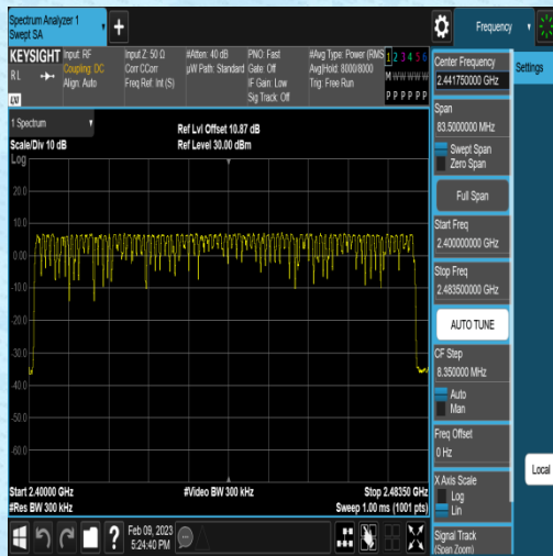
3DH5-Ant1-Hop
