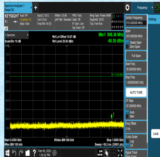
DH5-Ant1-2441-30~1000-6.14
