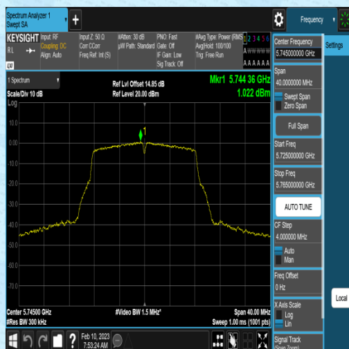
11A-Ant1-5745--1.35-0.15-2.22-0.00
