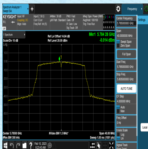
11N20SISO-Ant1-5785--2.36-0.13-2.22-0.00
