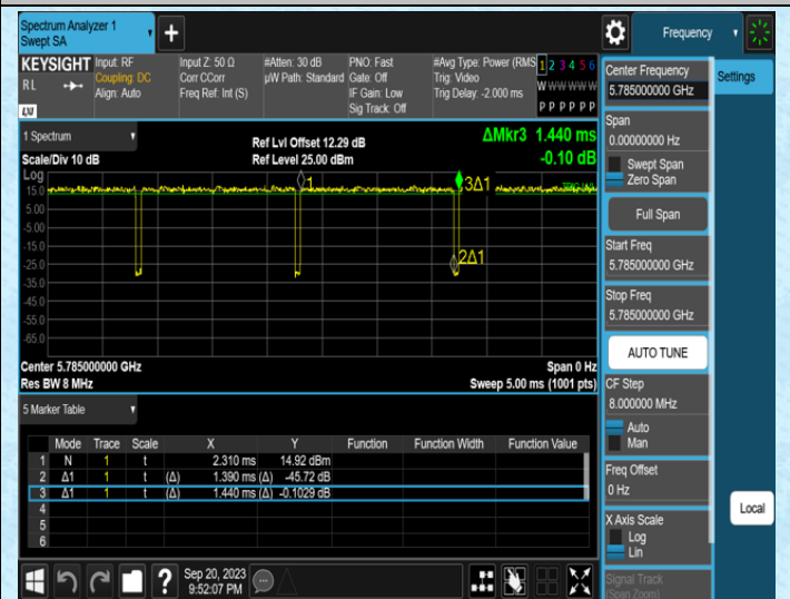
NTNV-11A-Ant1-5785
