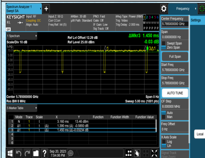
NTNV-11A-Ant0-5785
