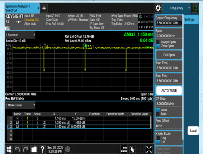
NTNV-11A-Ant1-5500
