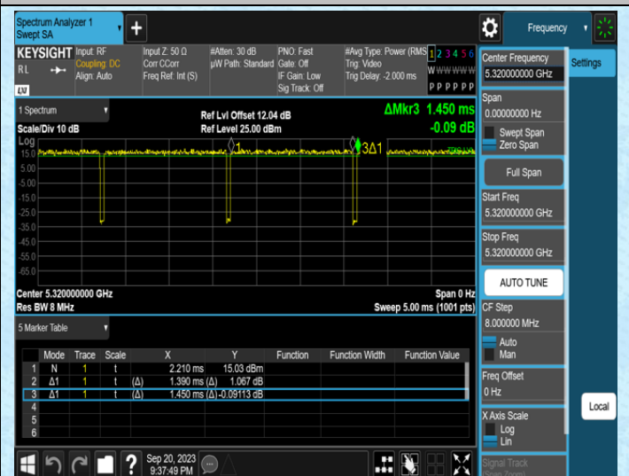
NTNV-11A-Ant1-5320
