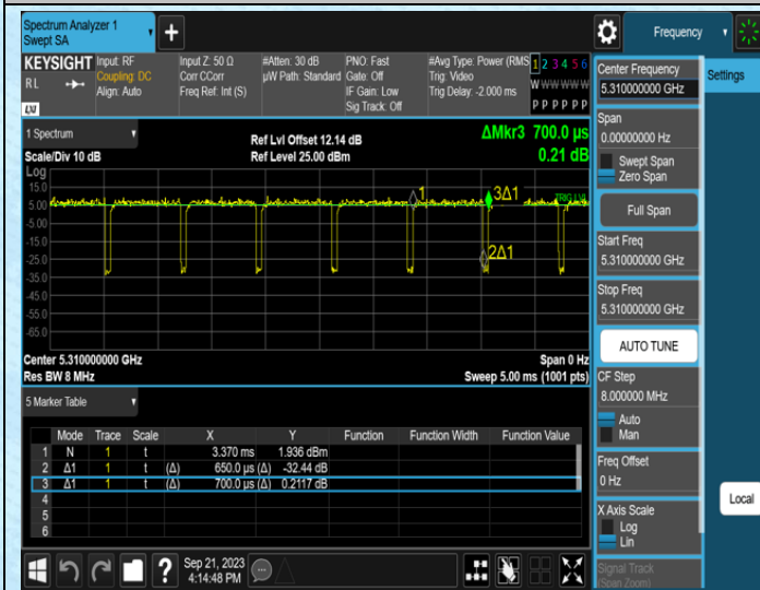
NTNV-11N40MIMO-Ant0-5310
