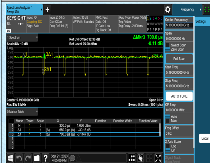
NTNV-11N40MIMO-Ant0-5190
