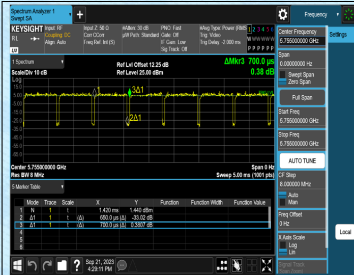
NTNV-11N40MIMO-Ant0-5755
