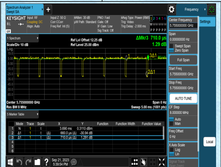
NTNV-11AC40MIMO-Ant1-5755
