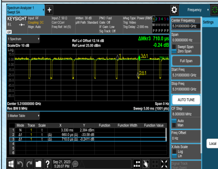
NTNV-11AC40MIMO-Ant0-5310
