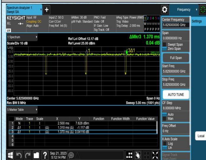
NTNV-11AC20MIMO-Ant0-5825
