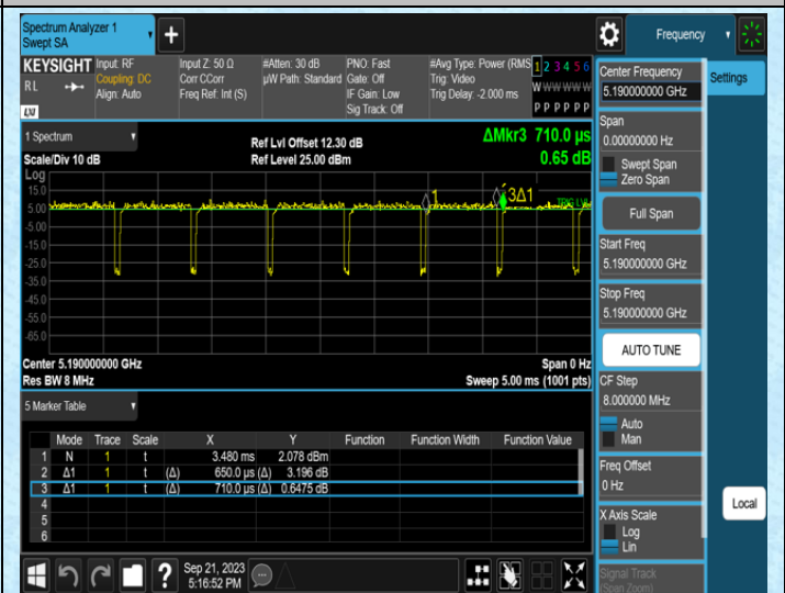
NTNV-11AC40MIMO-Ant1-5190
