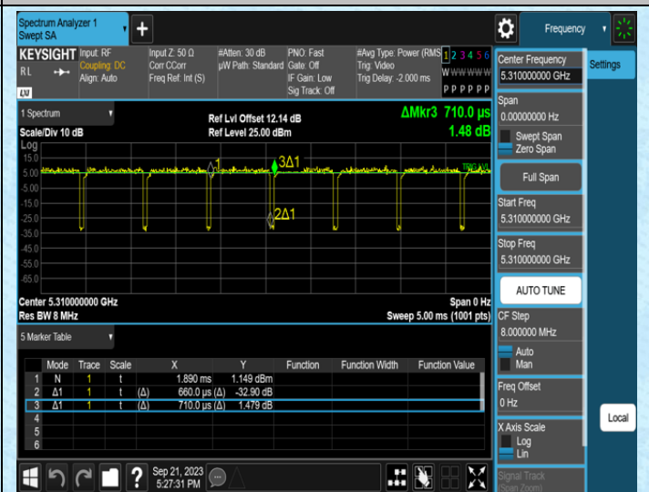
NTNV-11AC40MIMO-Ant1-5310
