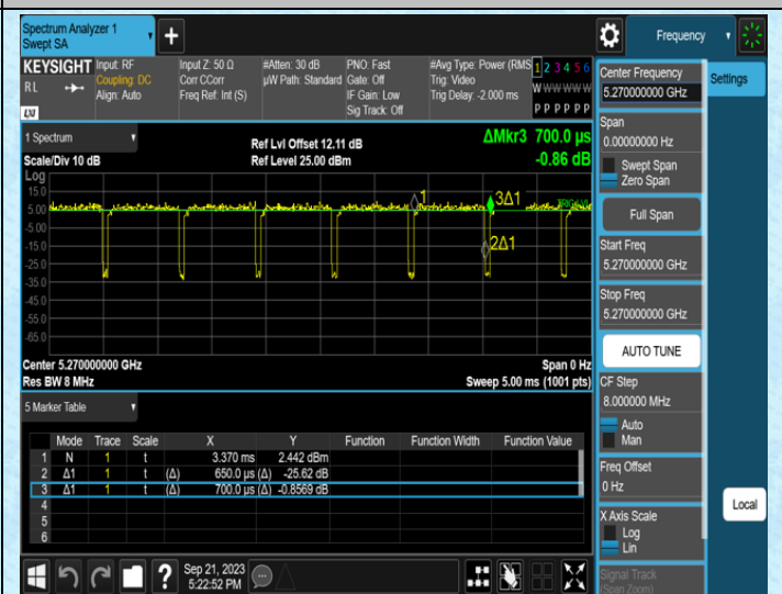
NTNV-11AC40MIMO-Ant1-5270
