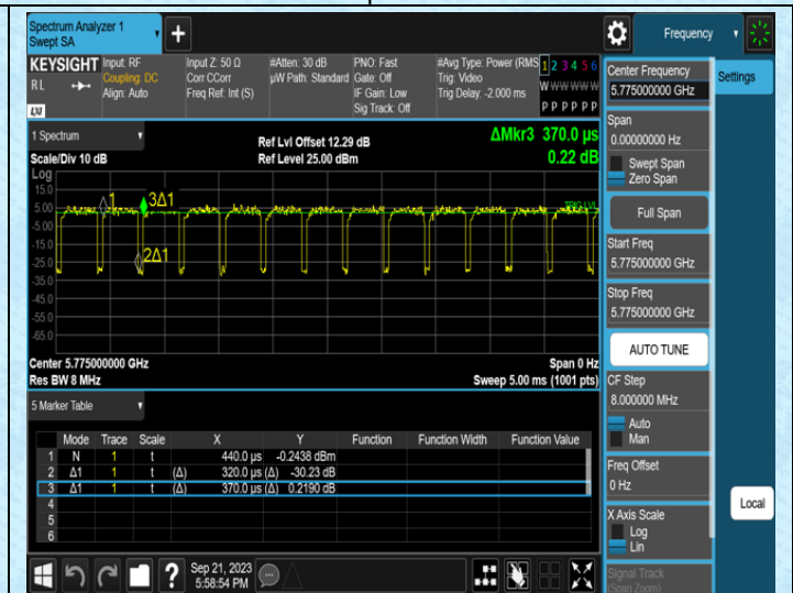
NTNV-11AC80MIMO-Ant1-5775
