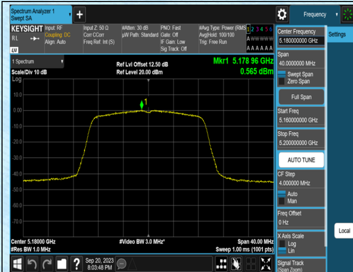
11N20SISO-Ant0-5180
