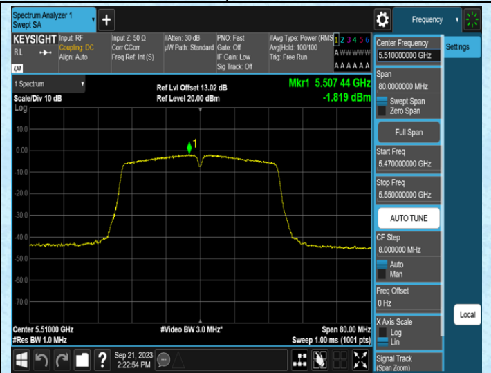
11N40SISO-Ant1-5510
