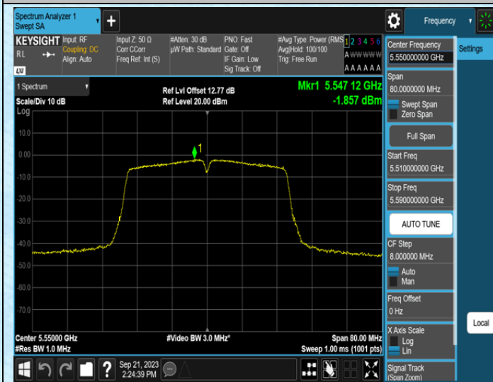
11N40SISO-Ant1-5550
