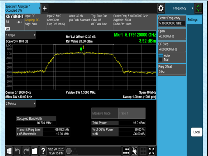
11A-Ant1-5180
