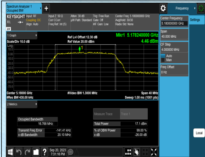
11A-Ant0-5180
