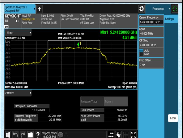
11A-Ant1-5240
