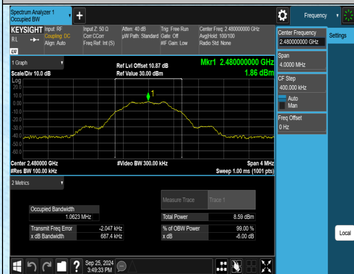
BLE_1M-Ant1-2480-PASS
