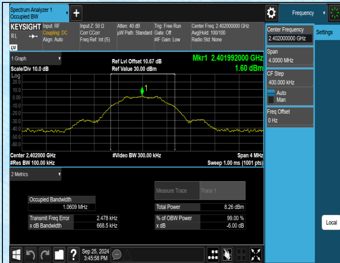
BLE_1M-Ant1-2402-PASS
