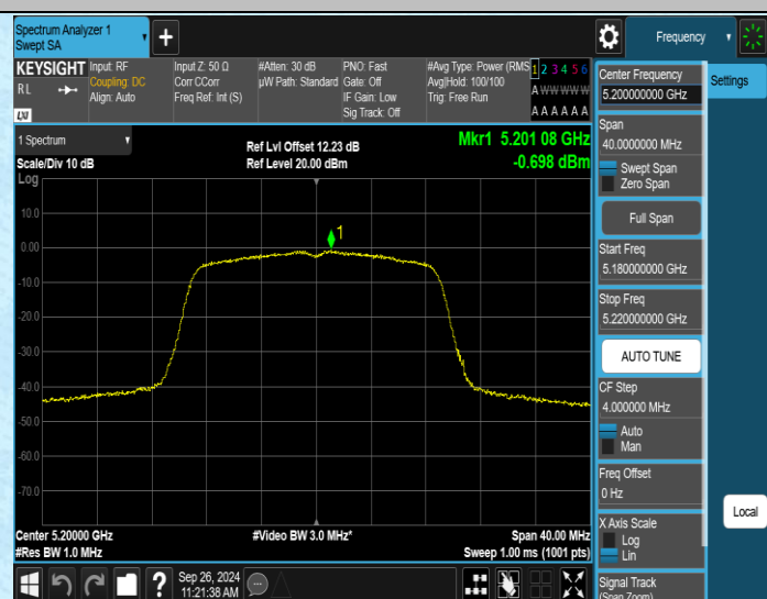
11AC20SISO-Ant2-5200-PASS
