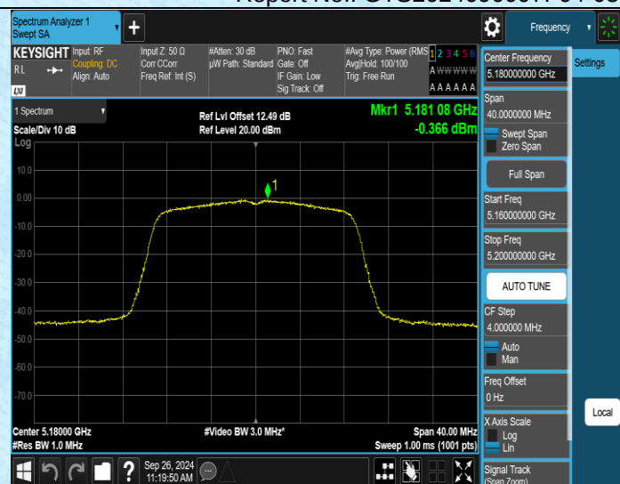
11AC20SISO-Ant2-5180-PASS
