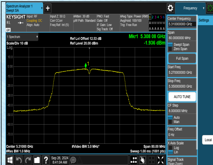
11N40SISO-Ant1-5310-PASS
