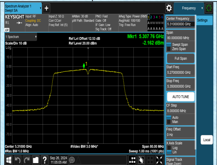
11N40SISO-Ant2-5310-PASS
