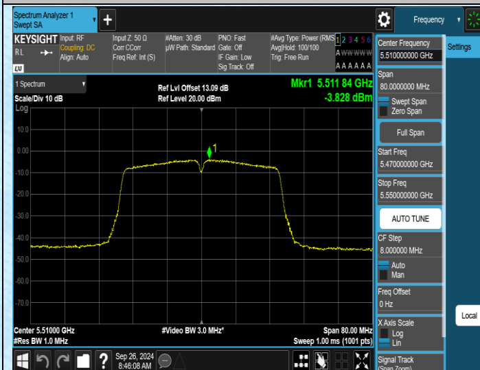
11N40SISO-Ant1-5510-PASS
