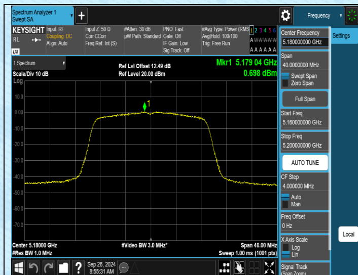
11AC20SISO-Ant1-5180-PASS
