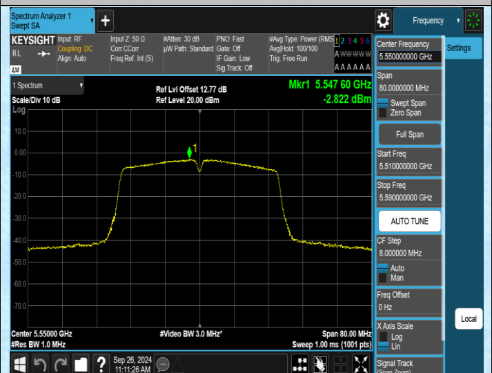
11N40SISO-Ant2-5550-PASS
