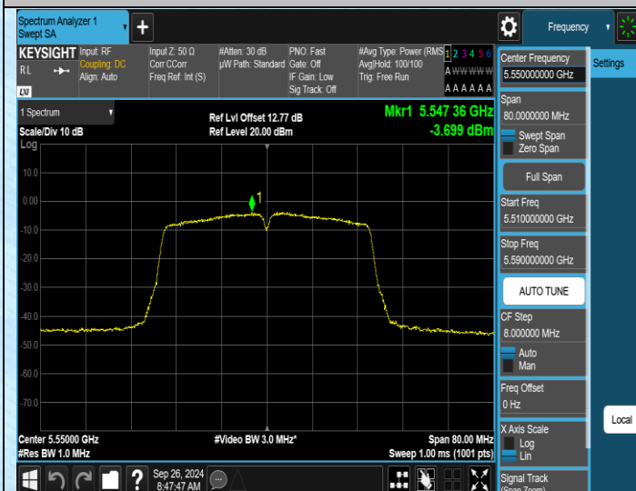
11N40SISO-Ant1-5550-PASS
