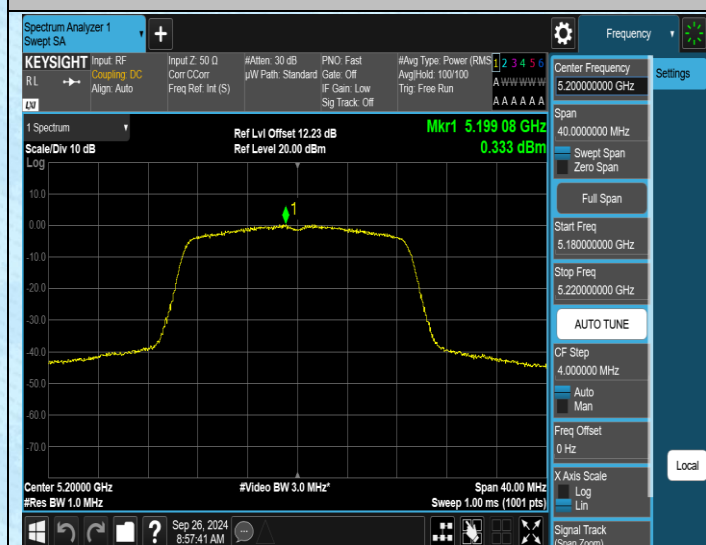
11AC20SISO-Ant1-5200-PASS
