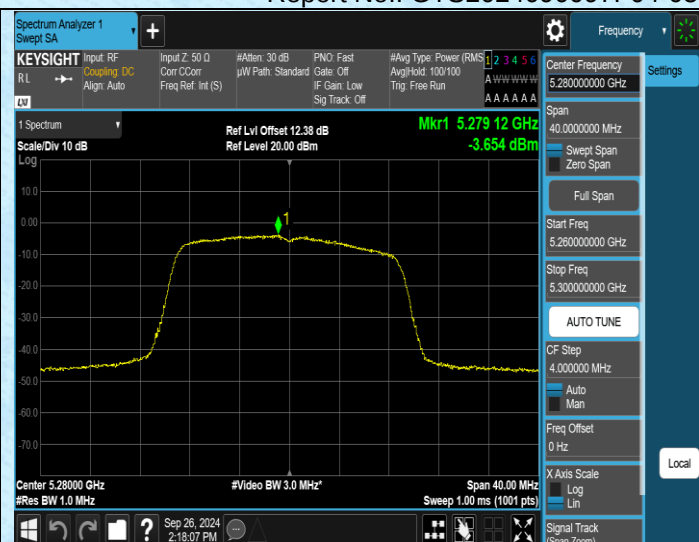
11N20MIMO-Ant2-5280-PASS
