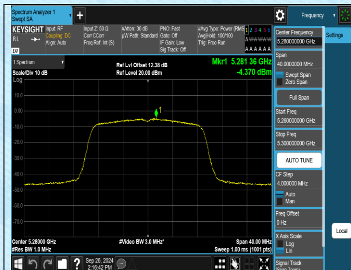
11N20MIMO-Ant1-5280-PASS
