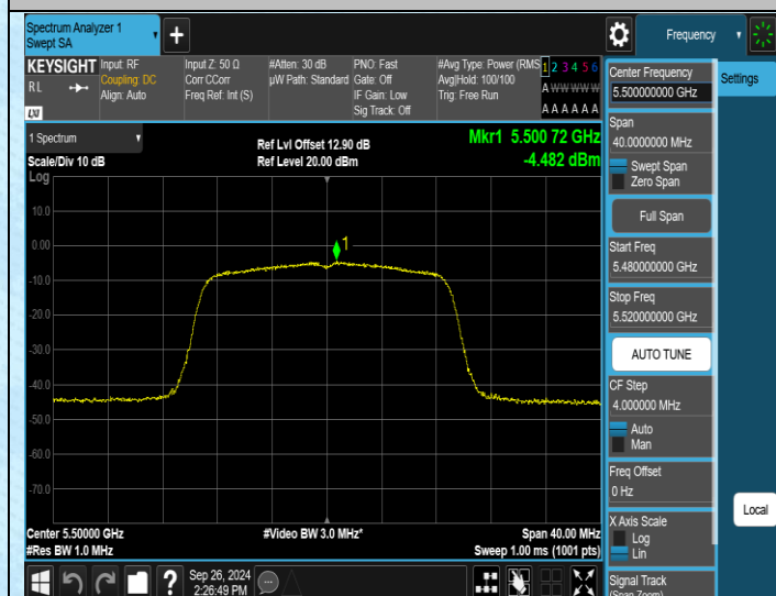
11N20MIMO-Ant1-5500-PASS
