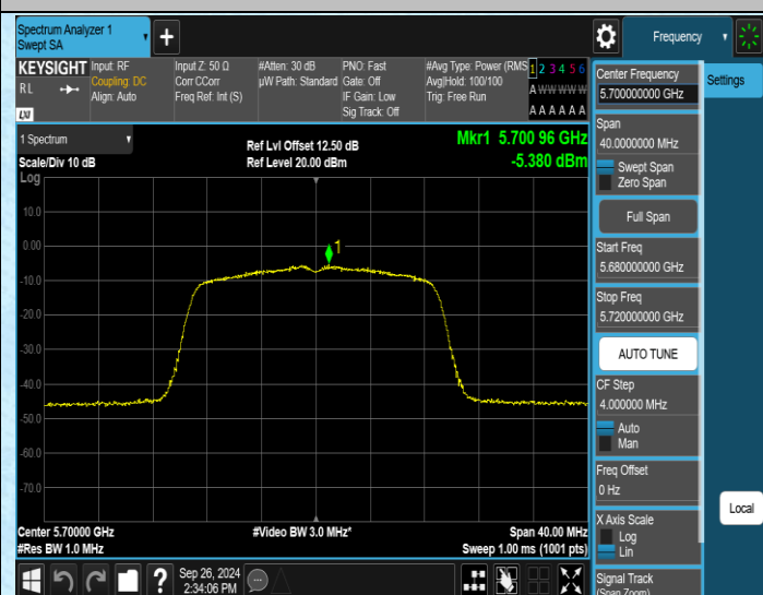
11N20MIMO-Ant2-5700-PASS
