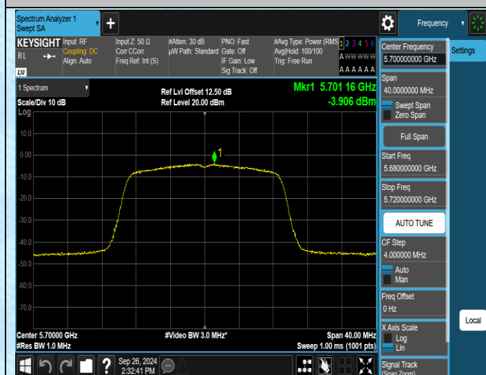
11N20MIMO-Ant1-5700-PASS
