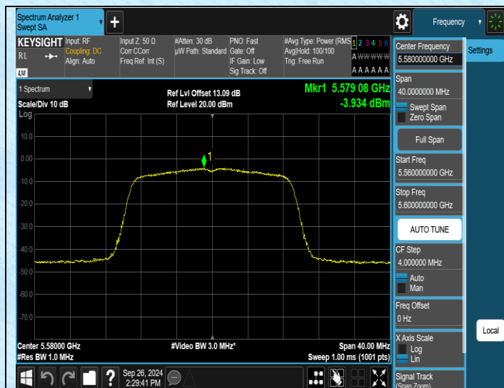
11N20MIMO-Ant1-5580-PASS
