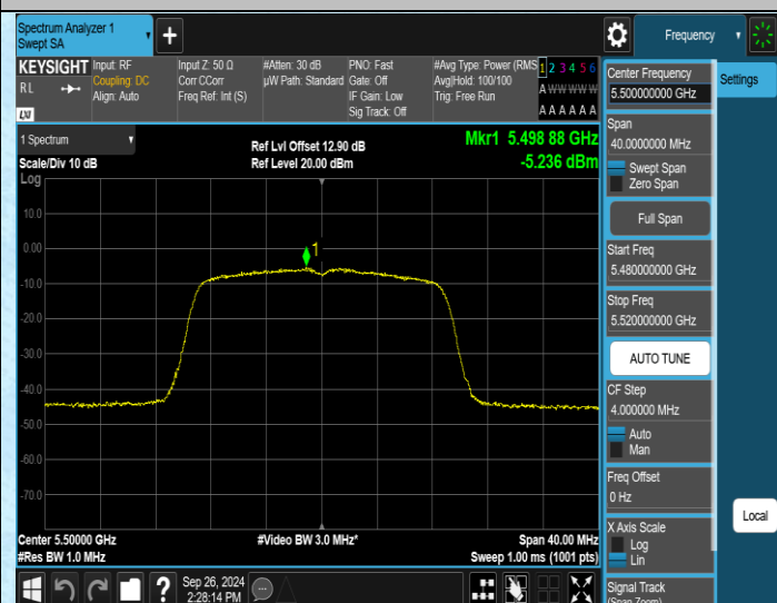
11N20MIMO-Ant2-5500-PASS
