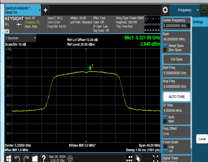
11N20MIMO-Ant2-5320-PASS
