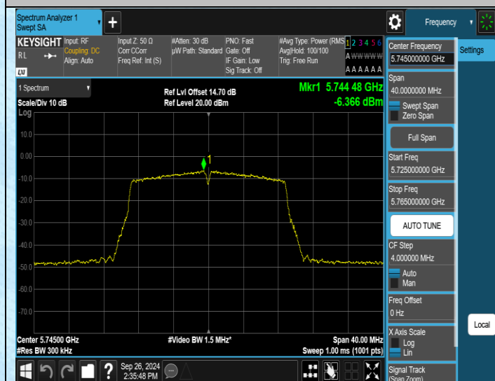
11N20MIMO-Ant1-5745-PASS
