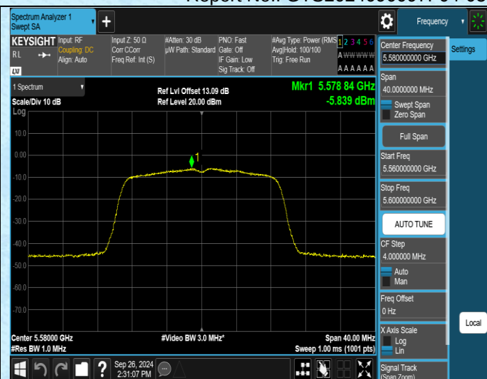
11N20MIMO-Ant2-5580-PASS
