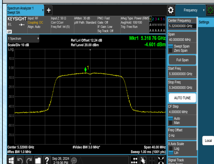
11N20MIMO-Ant1-5320-PASS
