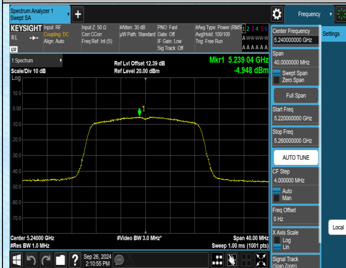
11N20MIMO-Ant1-5240-PASS
