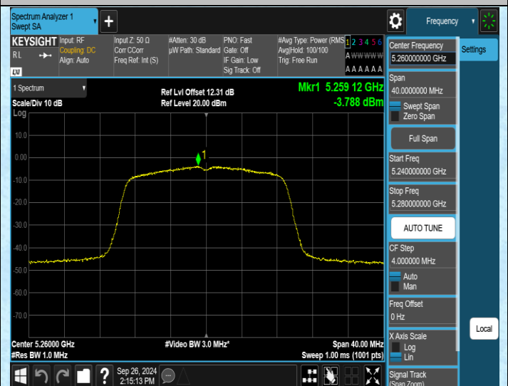
11N20MIMO-Ant2-5260-PASS
