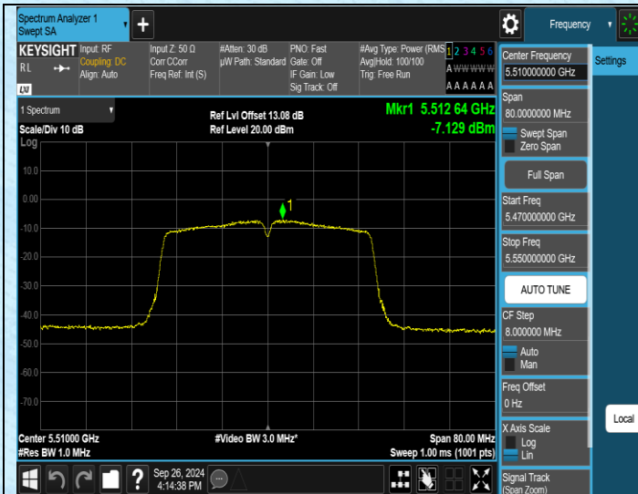
11AC40MIMO-Ant1-5510-PASS
