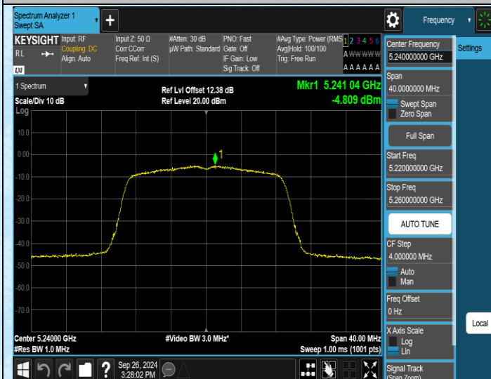
11AC20MIMO-Ant1-5240-PASS
