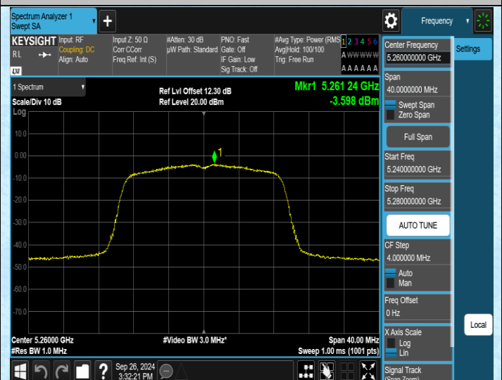
11AC20MIMO-Ant2-5260-PASS
