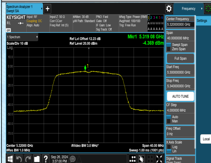
11AC20MIMO-Ant1-5320-PASS
