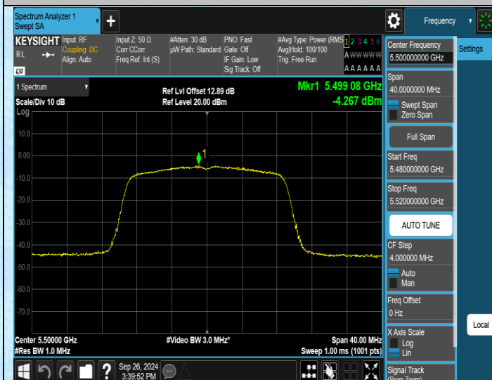
11AC20MIMO-Ant1-5500-PASS
