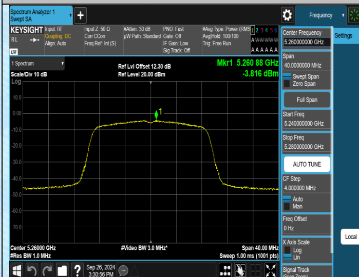
11AC20MIMO-Ant1-5260-PASS
