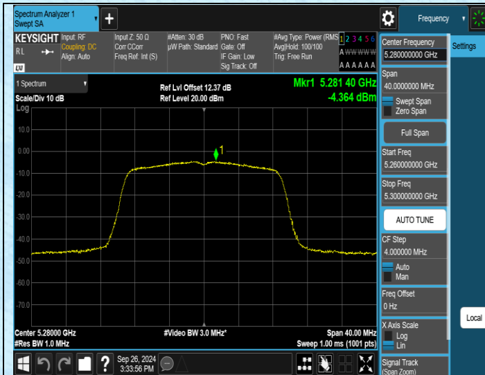
11AC20MIMO-Ant1-5280-PASS
