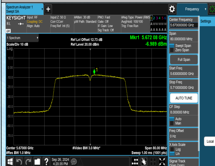
11AC40MIMO-Ant1-5670-PASS
