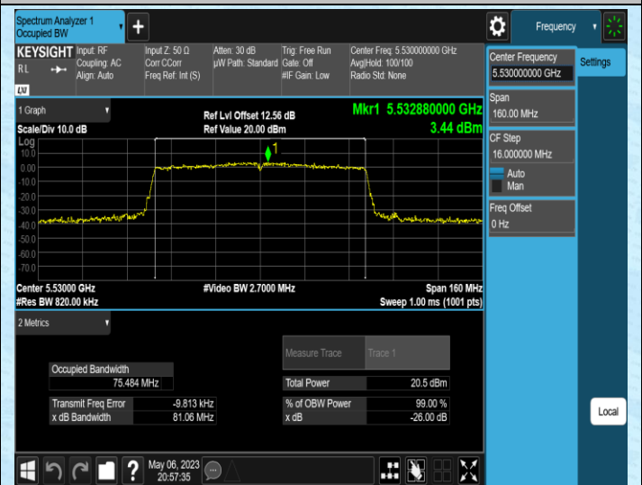
11AC80MIMO-Ant1-5530
