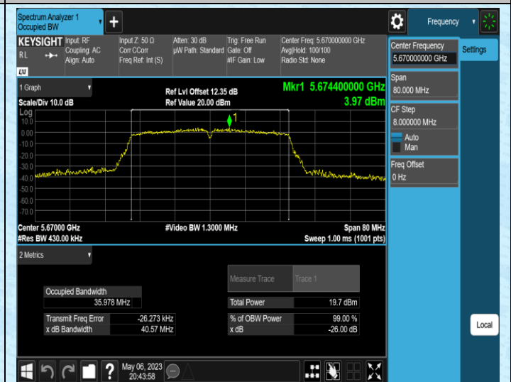
11AC40MIMO-Ant1-5670
