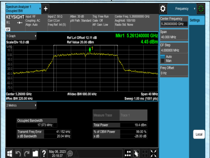
11AC20MIMO-Ant2-5260
