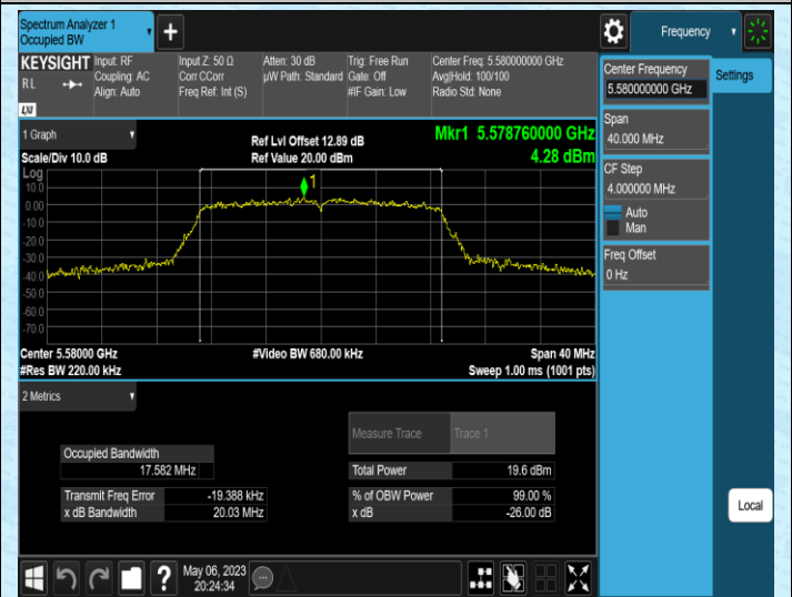
11AC20MIMO-Ant1-5580
