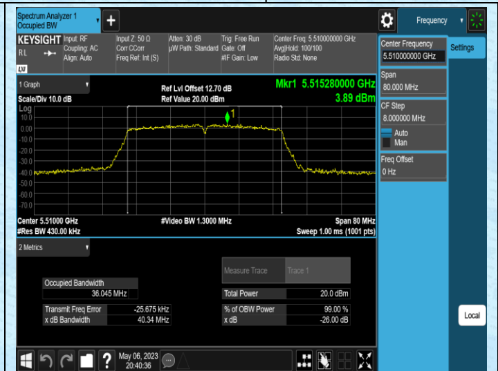
11AC40MIMO-Ant1-5510
