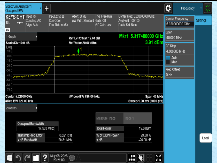
11AC20MIMO-Ant1-5320
