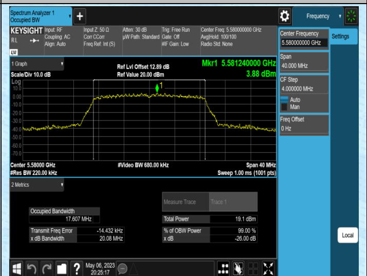
11AC20MIMO-Ant2-5580
