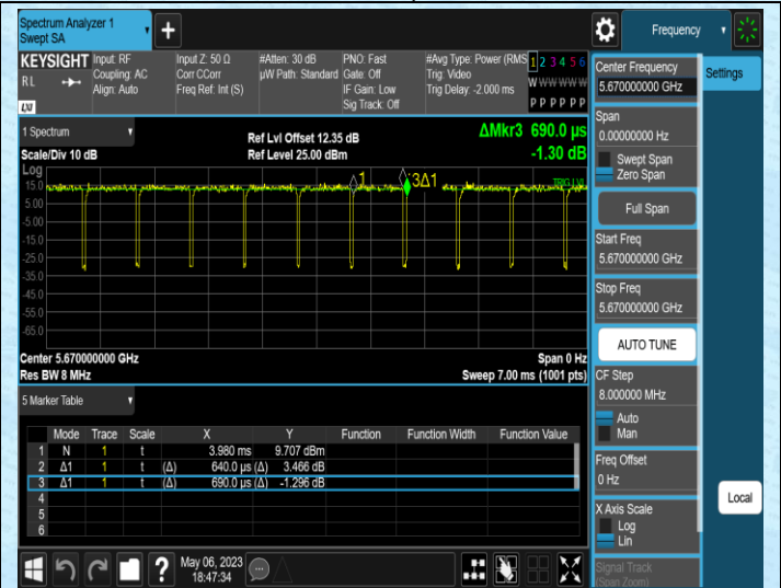
NTNV-11N40SISO-Ant2-5670
