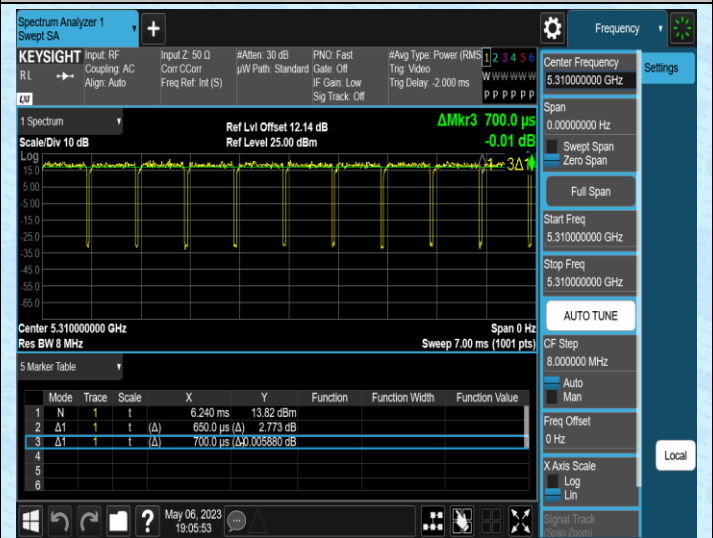
NTNV-11AC40SISO-Ant2-5310
