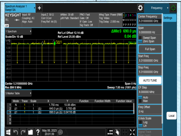
NTNV-11N40MIMO-Ant2-5310
