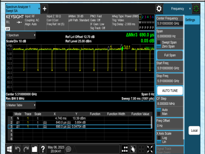
NTNV-11N40MIMO-Ant2-5510
