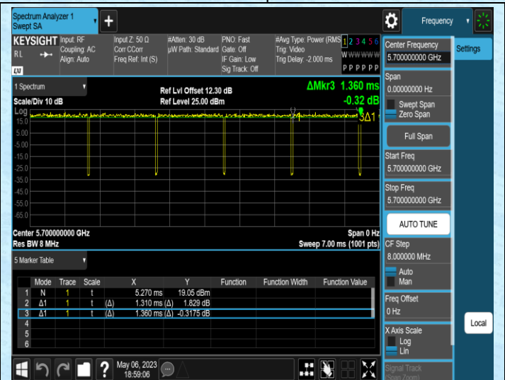
NTNV-11AC20SISO-Ant2-5700
