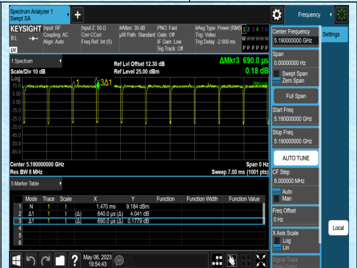
NTNV-11N40MIMO-Ant2-5190
