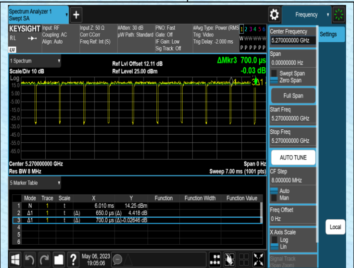
NTNV-11AC40SISO-Ant2-5270
