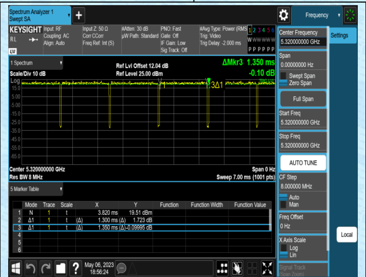
NTNV-11AC20SISO-Ant2-5320
