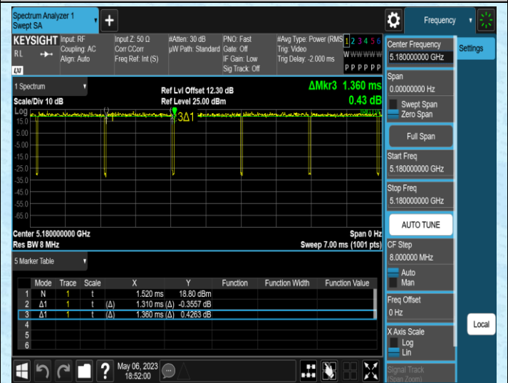
NTNV-11AC20SISO-Ant2-5180
