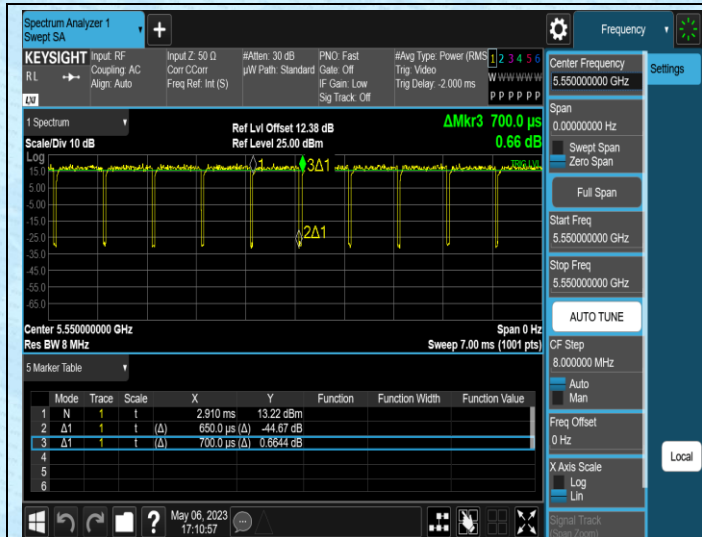
NTNV-11AC40SISO-Ant1-5550
