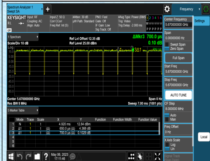
NTNV-11AC40SISO-Ant1-5670
