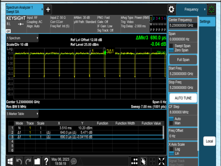
NTNV-11N40MIMO-Ant2-5230
