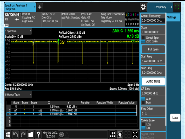
NTNV-11AC20SISO-Ant2-5240
