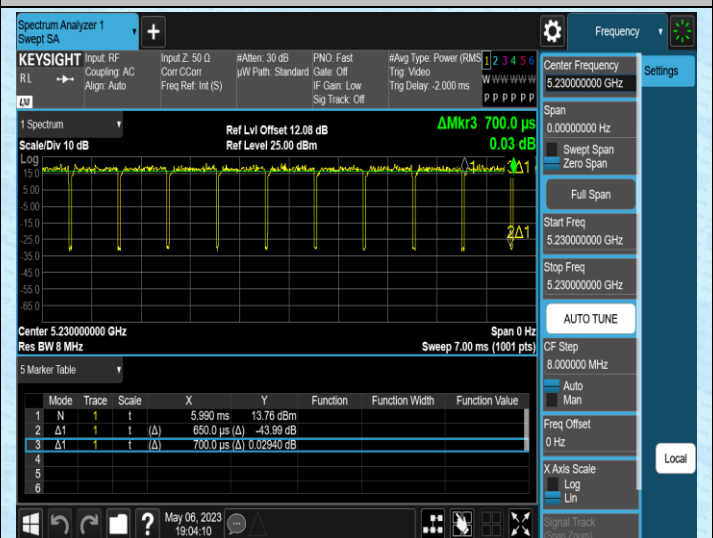
NTNV-11AC40SISO-Ant2-5230
