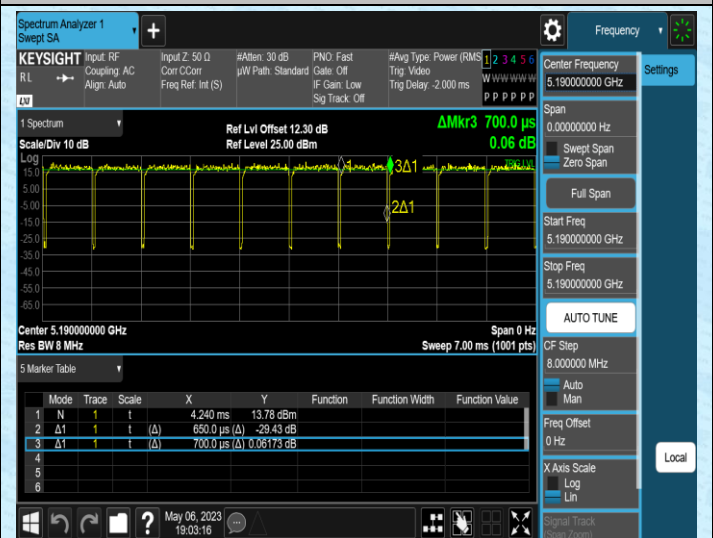
NTNV-11AC40SISO-Ant2-5190
