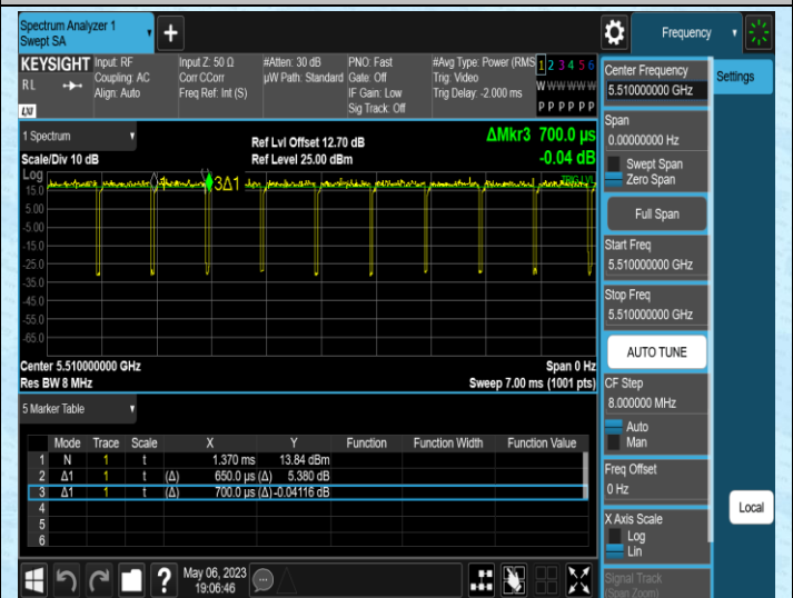
NTNV-11AC40SISO-Ant2-5510
