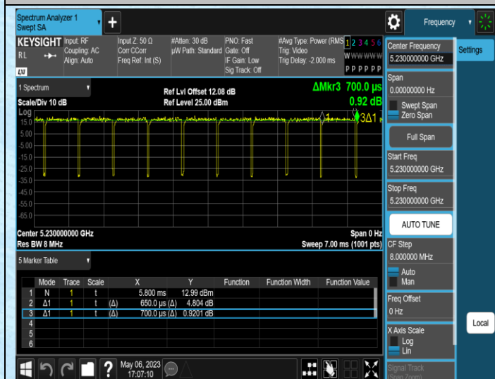
NTNV-11AC40SISO-Ant1-5230
