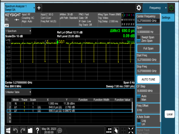
NTNV-11N40MIMO-Ant2-5270
