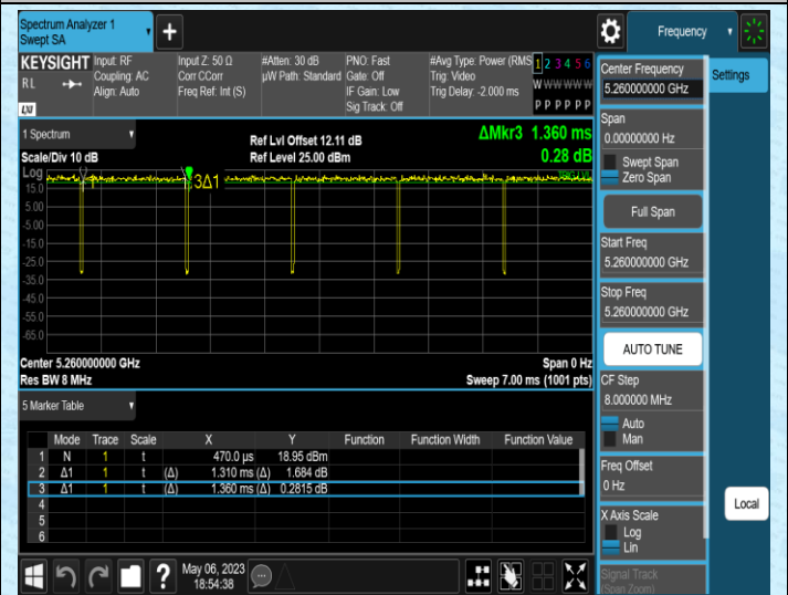
NTNV-11AC20SISO-Ant2-5260
