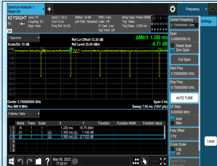
NTNV-11AC20SISO-Ant1-5700
