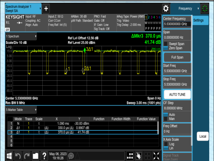
NTNV-11AC80SISO-Ant2-5530
