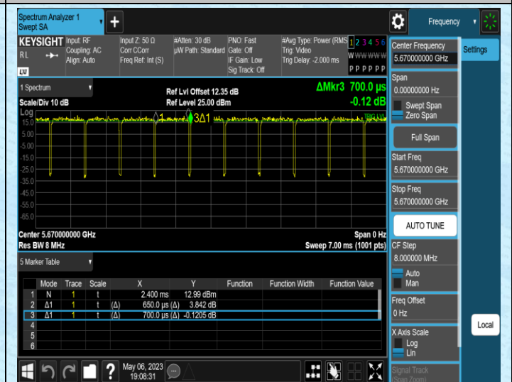
NTNV-11AC40SISO-Ant2-5670
