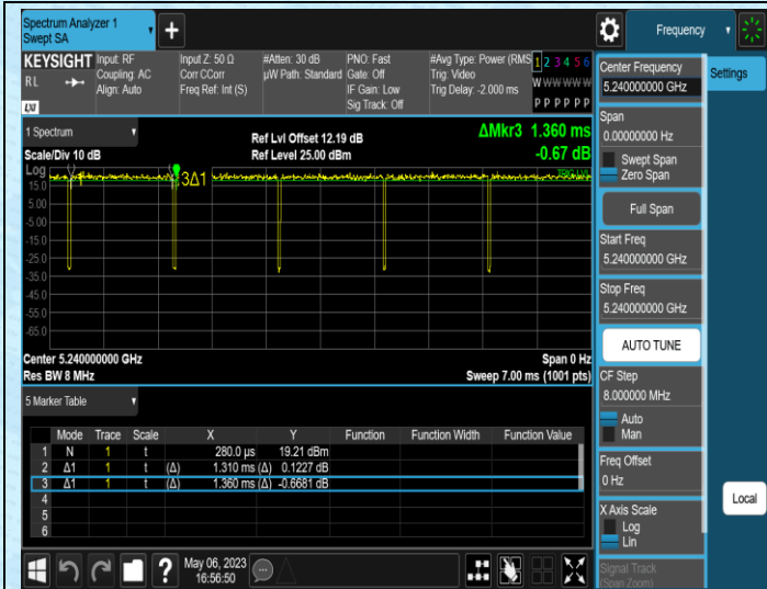
NTNV-11AC20SISO-Ant1-5240
