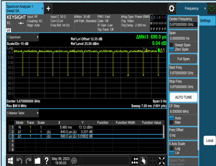
NTNV-11N40SISO-Ant1-5670
