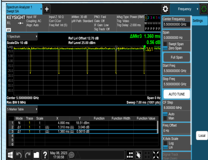
NTNV-11AC20SISO-Ant1-5500
