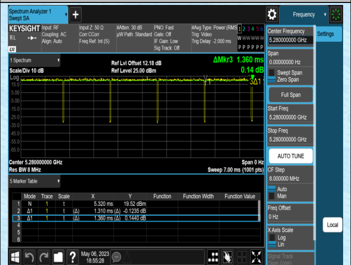
NTNV-11AC20SISO-Ant2-5280
