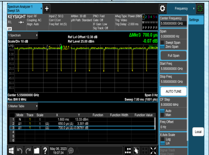
NTNV-11AC40SISO-Ant2-5550
