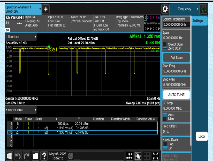
NTNV-11AC20SISO-Ant2-5500
