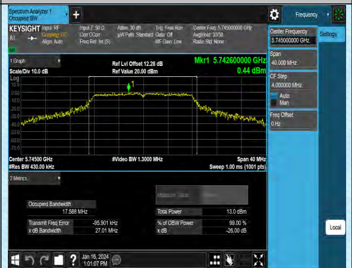
11A-Ant2-5745
