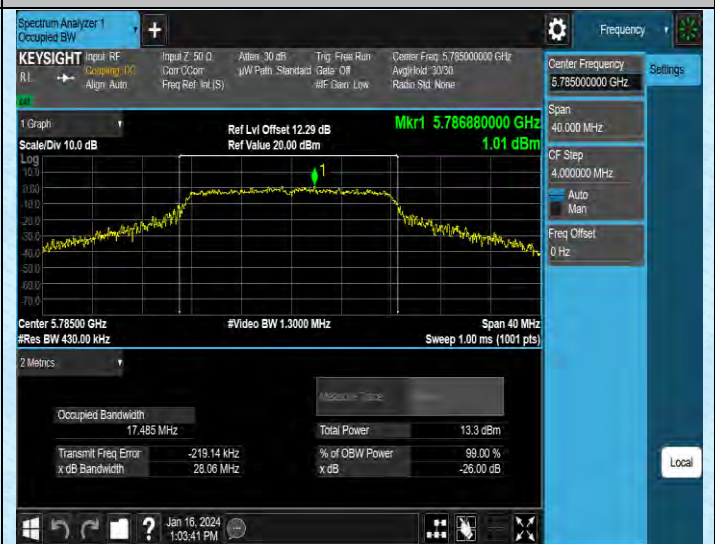
11A-Ant2-5785
