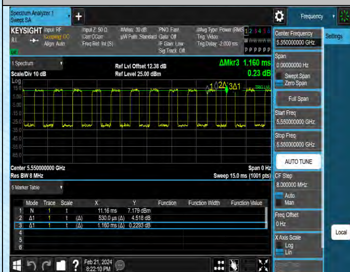
NTNV-11AX40SISO-Ant1-5550
