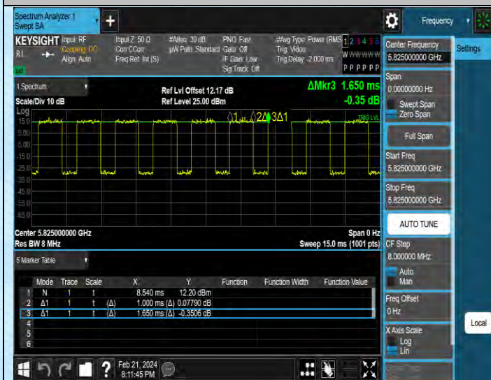
NTNV-11AX20SISO-Ant1-5825
