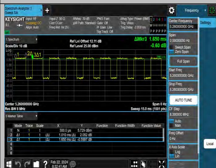
NTNV-11AX20MIMO-Ant2-5260
