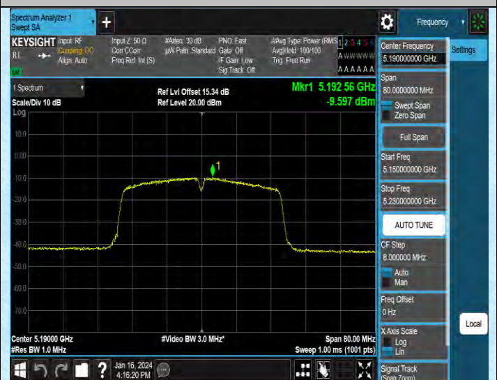
11N40MIMO-Ant2-5190-PASS
