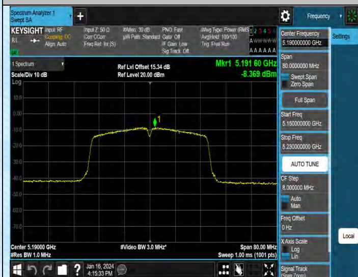
11N40MIMO-Ant1-5190-PASS
