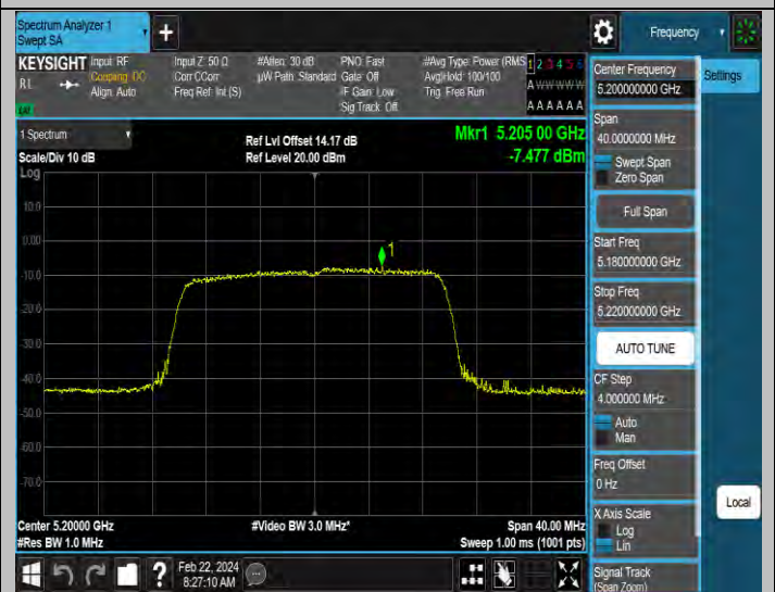
11AX20MIMO-Ant2-5200-PASS
