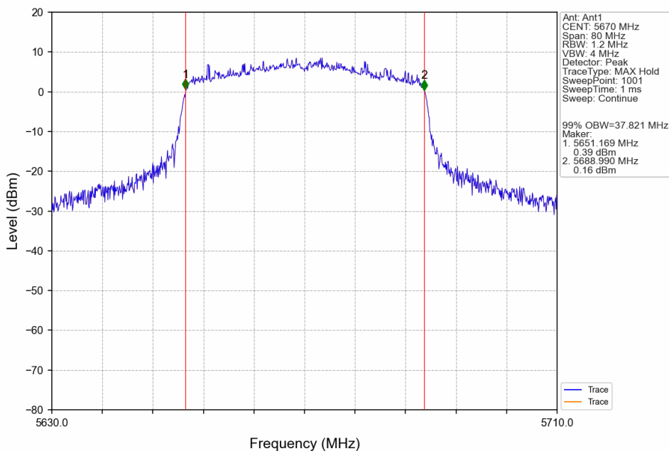
802.11ax(HEW40)_HCH_5670MHz_SU_/_Ant1_NTNV
