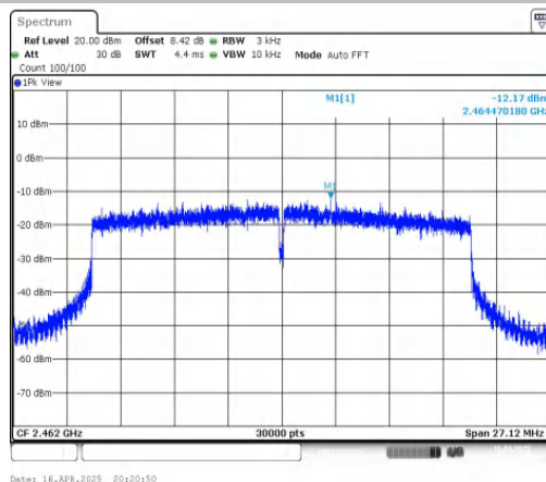
11AX20MIMO-Ant2-2462-PASS
