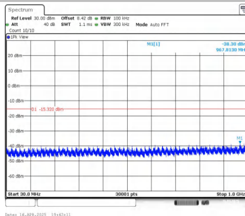
11N20MIMO-Ant2-2437-30~1000-PASS
