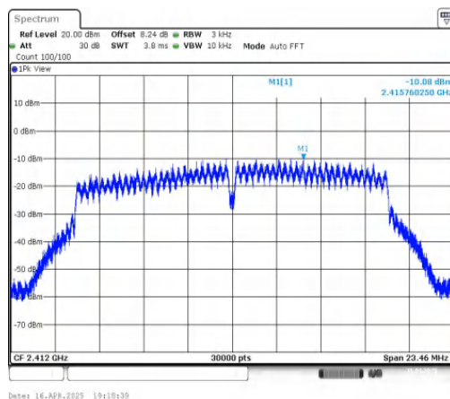
11G-CDD-Ant2-2412-PASS
