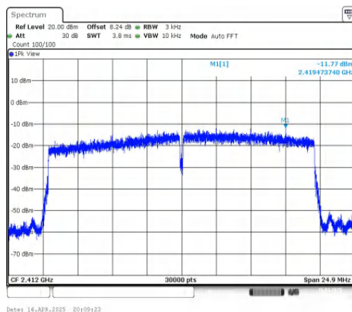
11AX20MIMO-Ant2-2412-PASS
