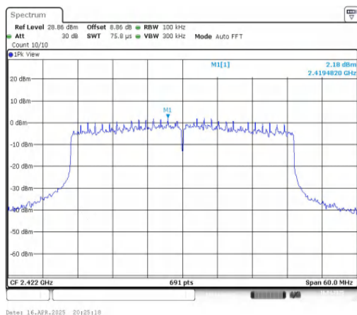
11AX40MIMO-Ant1-2422-0~Reference-PASS
