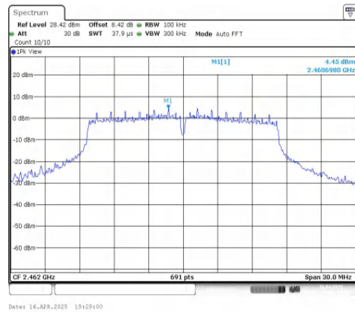
11G-CDD-Ant2-2462-0~Reference-PASS
