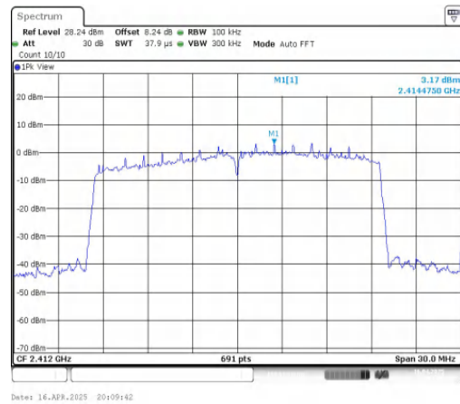
11AX20MIMO-Ant2-2412-0~Reference-PASS
