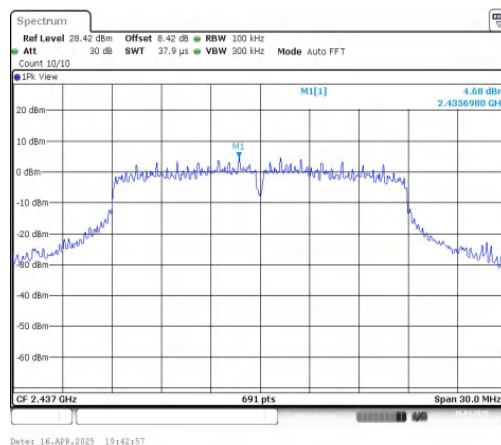
11N20MIMO-Ant2-2437-0~Reference-PASS
