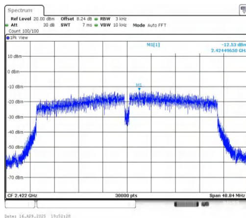
11N40MIMO-Ant2-2422-PASS
