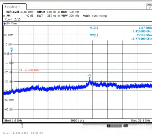
11N40MIMO-Ant1-2422-1000~26500-PASS
