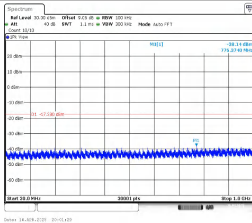
11N40MIMO-Ant1-2452-30~1000-PASS
