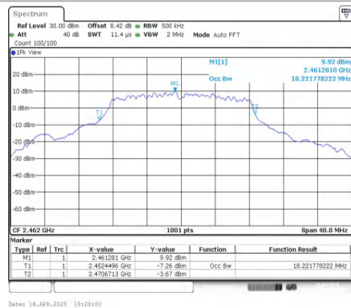
11G-CDD-Ant2-2462
