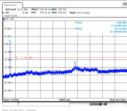
11N40MIMO-Ant1-2437-1000~26500-PASS
