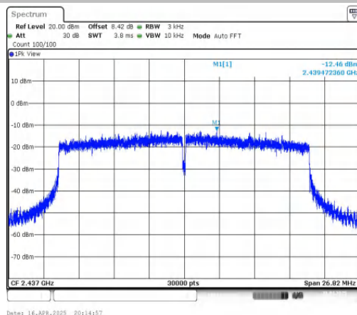
11AX20MIMO-Ant2-2437-PASS
