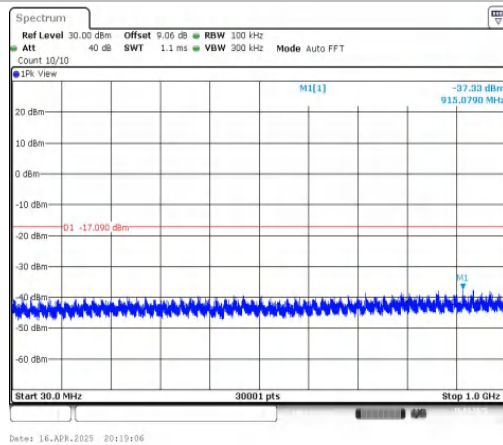
11AX20MIMO-Ant1-2462-30~1000-PASS
