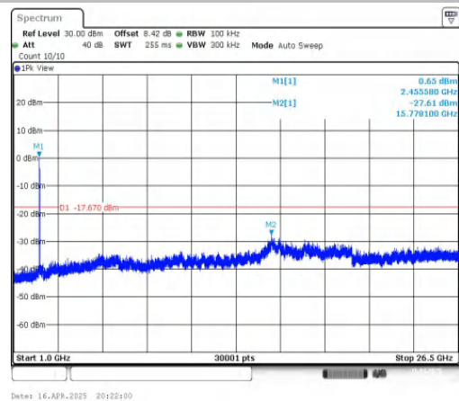
11AX20MIMO-Ant2-2462-1000~26500-PASS
