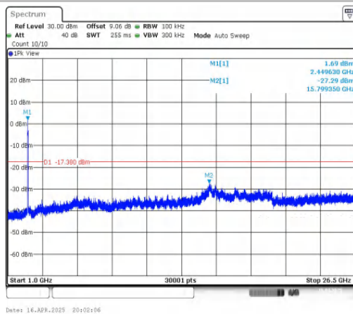
11N40MIMO-Ant1-2452-1000~26500-PASS
