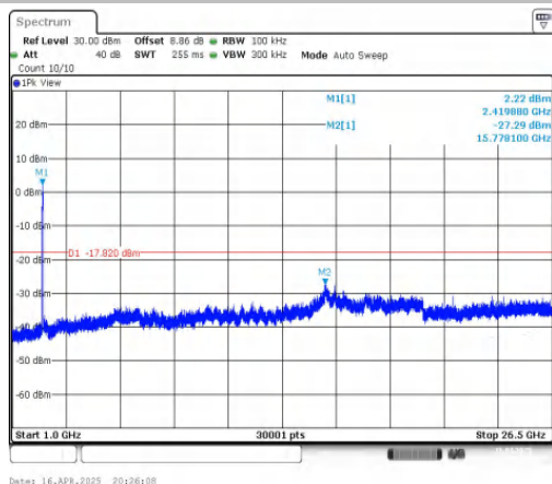
11AX40MIMO-Ant1-2422-1000~26500-PASS
