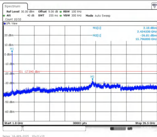
11AX40MIMO-Ant1-2437-1000~26500-PASS
