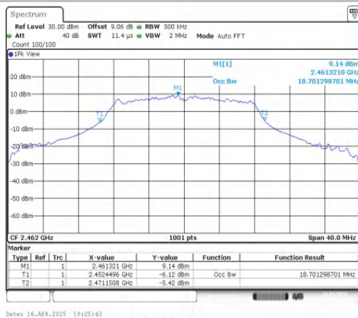
11G-CDD-Ant1-2462
