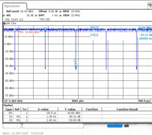
NTNV-11G-CDD-Ant1-2462
