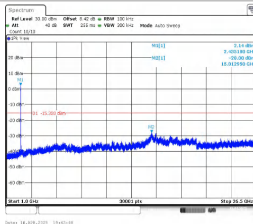
11N20MIMO-Ant2-2437-1000~26500-PASS
