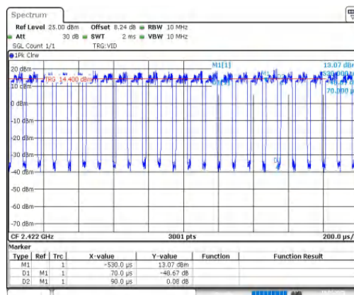
NTNV-11AX40MIMO-Ant2-2422
