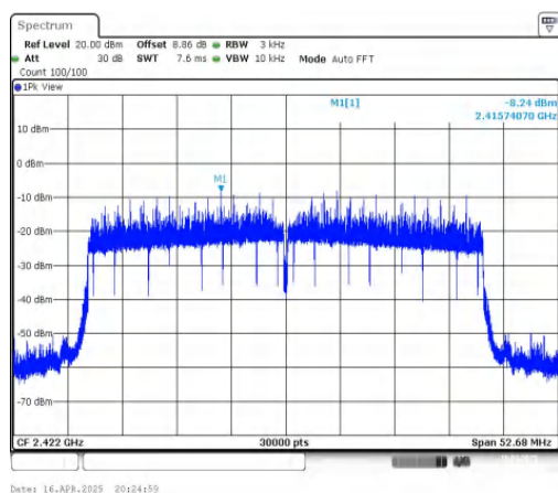
11AX40MIMO-Ant1-2422-PASS
