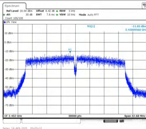
11N40MIMO-Ant2-2452-PASS
