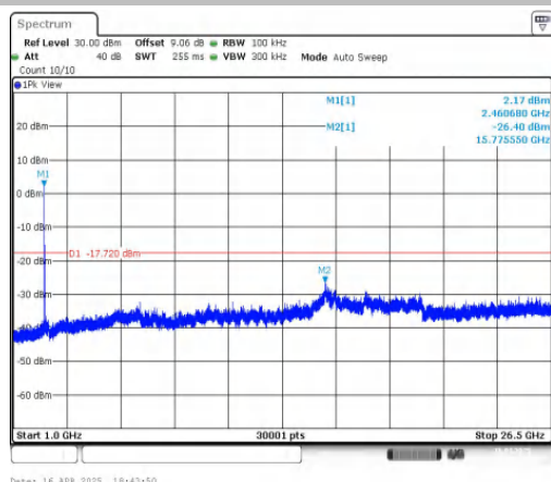
11B-CDD-Ant1-2462-1000~26500-PASS
