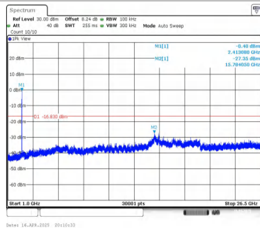
11AX20MIMO-Ant2-2412-1000~26500-PASS
