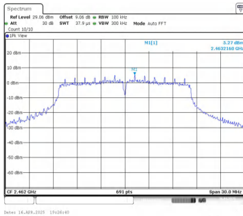
11G-CDD-Ant1-2462-0~Reference-PASS
