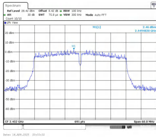
11N40MIMO-Ant2-2452-0~Reference-PASS
