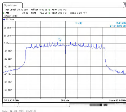
11AX40MIMO-Ant2-2437-0~Reference-PASS
