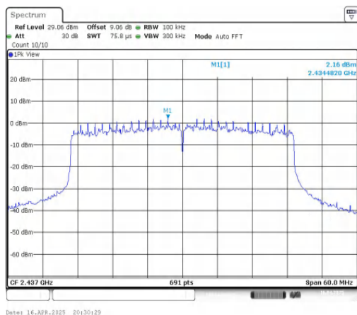
11AX40MIMO-Ant1-2437-0~Reference-PASS
