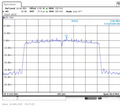
11AX20MIMO-Ant1-2412-0~Reference-PASS
