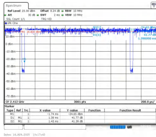
NTNV-11G-CDD-Ant2-2412
