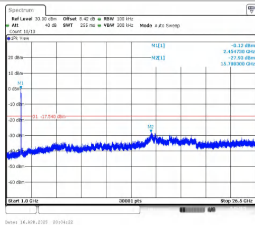
11N40MIMO-Ant2-2452-1000~26500-PASS
