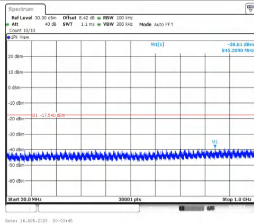
11N40MIMO-Ant2-2452-30~1000-PASS
