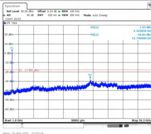
11AX40MIMO-Ant2-2422-1000~26500-PASS
