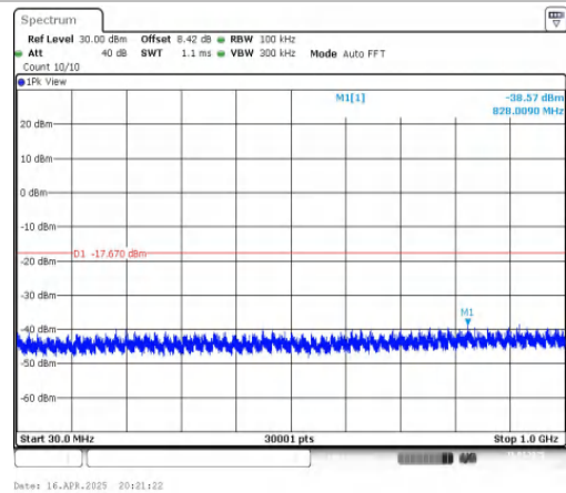
11AX20MIMO-Ant2-2462-30~1000-PASS
