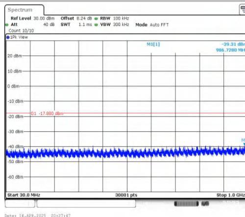
11AX40MIMO-Ant2-2422-30~1000-PASS
