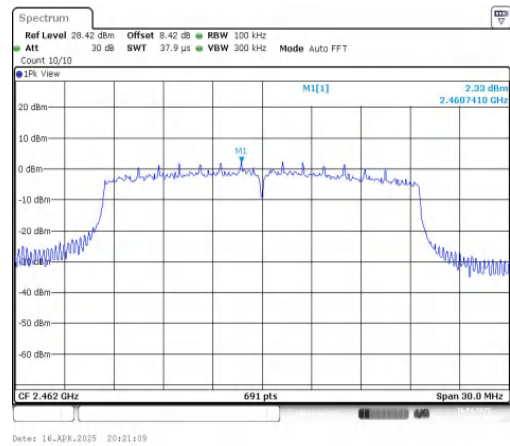
11AX20MIMO-Ant2-2462-0~Reference-PASS
