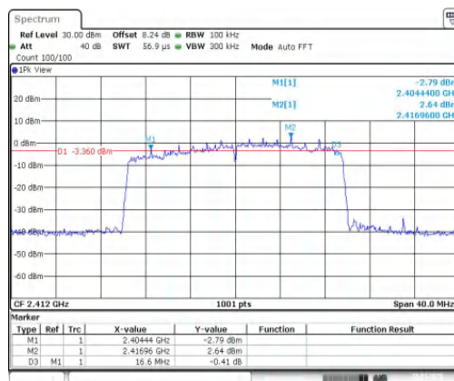
11AX20MIMO-Ant2-2412-PASS
