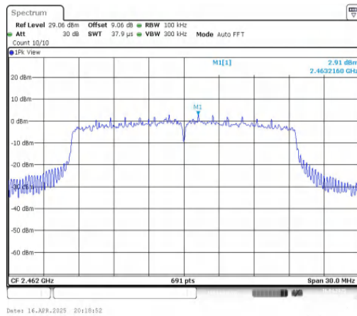
11AX20MIMO-Ant1-2462-0~Reference-PASS
