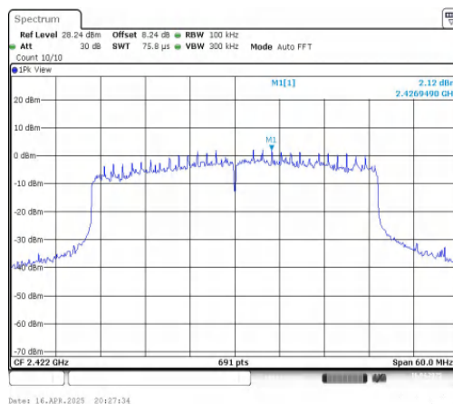
11AX40MIMO-Ant2-2422-0~Reference-PASS
