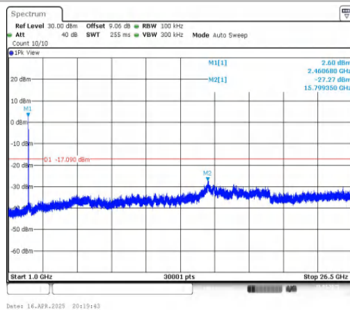
11AX20MIMO-Ant1-2462-1000~26500-PASS
