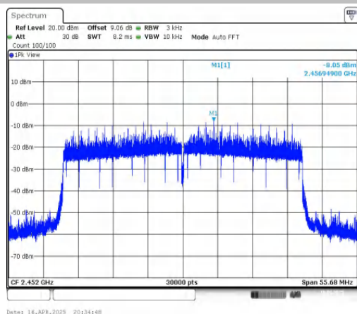
11AX40MIMO-Ant1-2452-PASS
