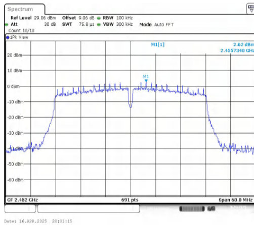
11N40MIMO-Ant1-2452-0~Reference-PASS
