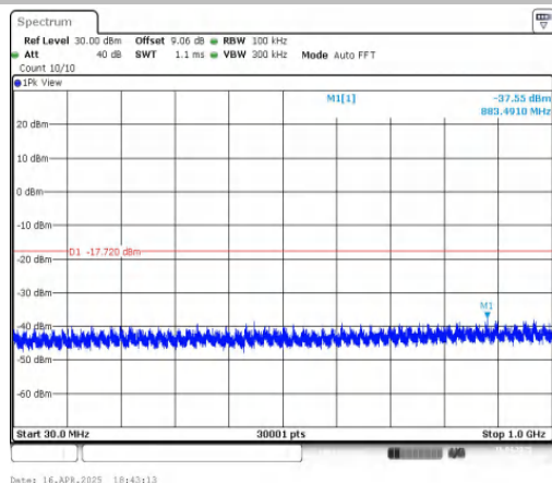
11B-CDD-Ant1-2462-30~1000-PASS
