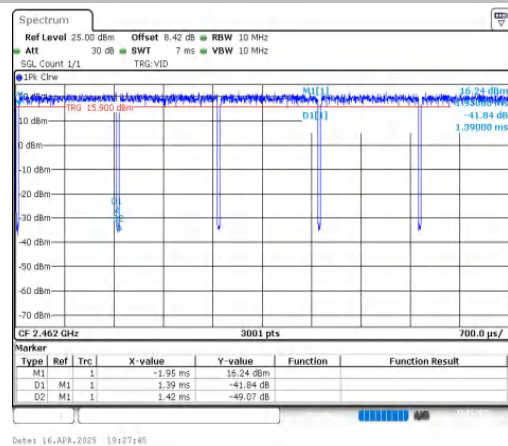
NTNV-11G-CDD-Ant2-2462
