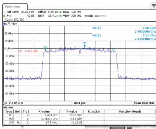
11AX20MIMO-Ant1-2412-PASS
