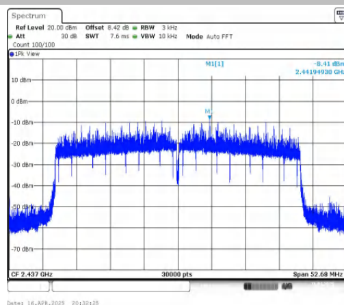
11AX40MIMO-Ant2-2437-PASS
