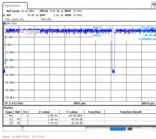
NTNV-11G-CDD-Ant1-2412
