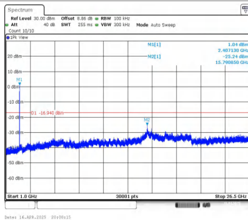
11AX20MIMO-Ant1-2412-1000~26500-PASS
