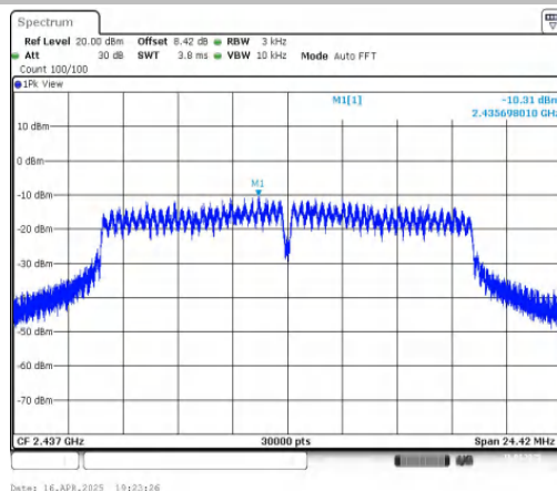
11G-CDD-Ant2-2437-PASS
