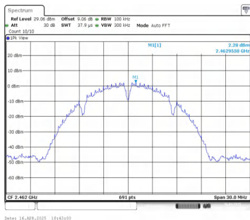
11B-CDD-Ant1-2462-0~Reference-PASS
