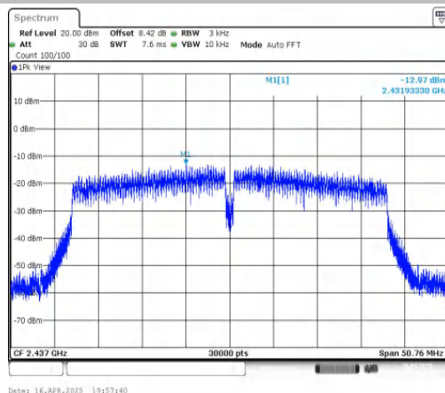
11N40MIMO-Ant2-2437-PASS
