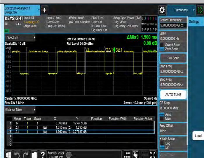
NTNV-11AC20SISO-Ant2-5700
