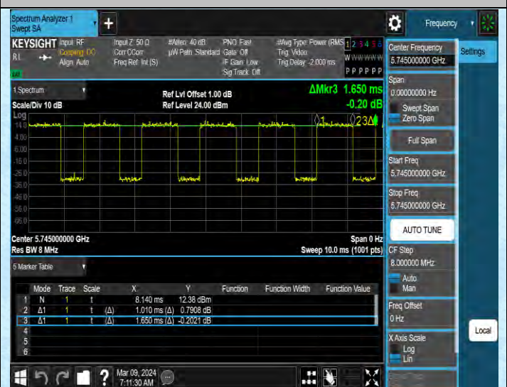
NTNV-11AX20SISO-Ant2-5745
