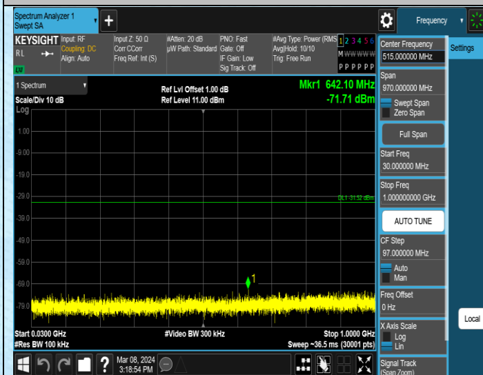
11AX20MIMO-Ant2-2437-30~1000-PASS
