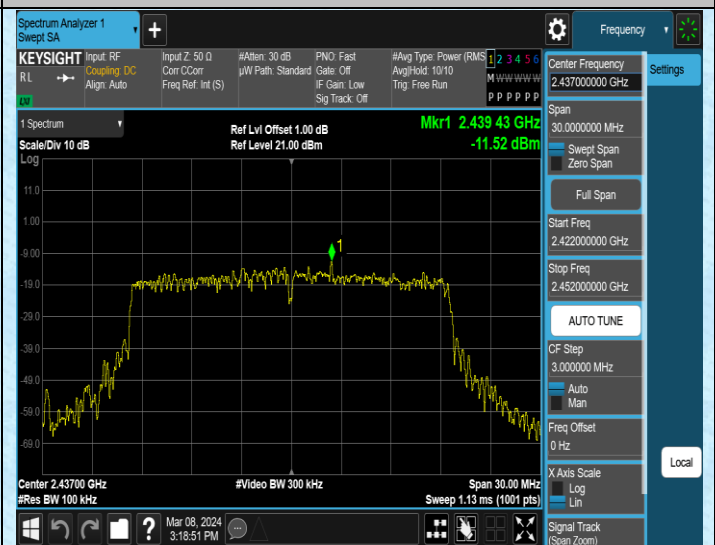
11AX20MIMO-Ant2-2437-0-Reference-PASS
