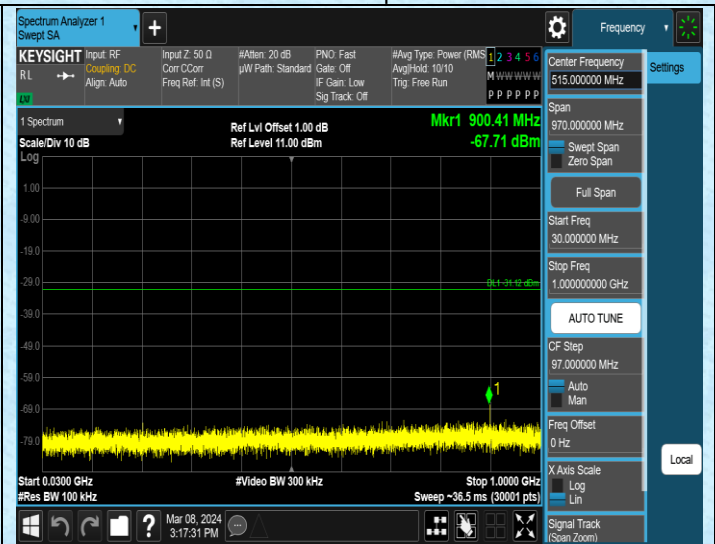
11AX20MIMO-Ant1-2437-30~1000-PASS
