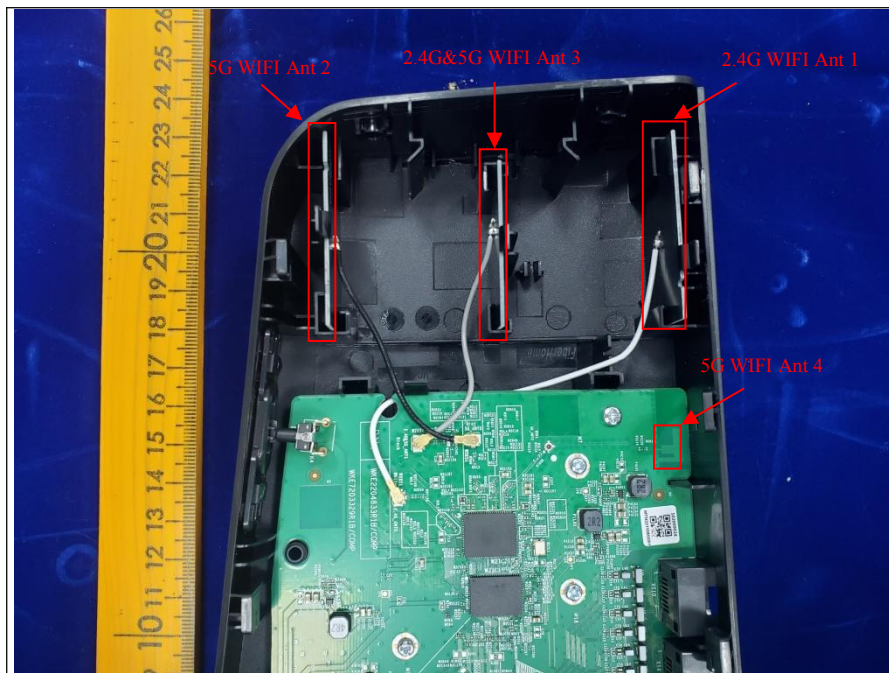
EUT-antenna
