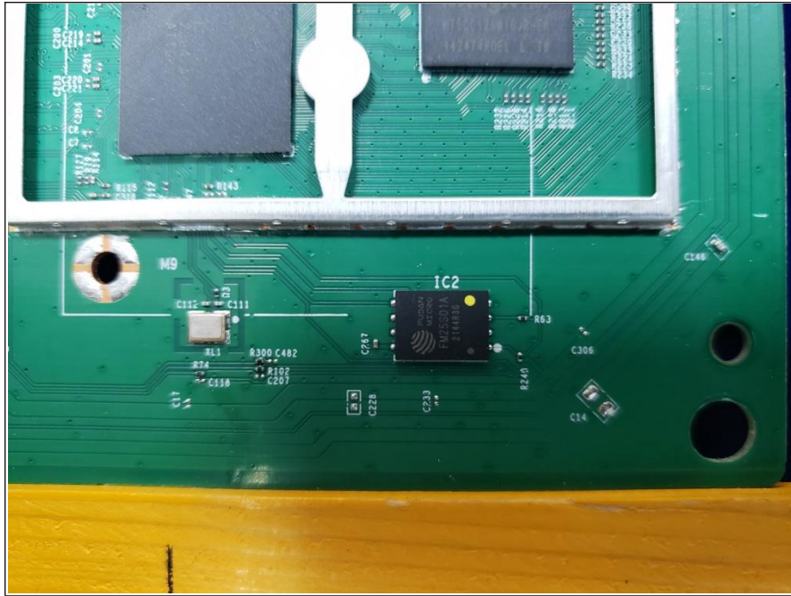
SR1021FS EUT-9
