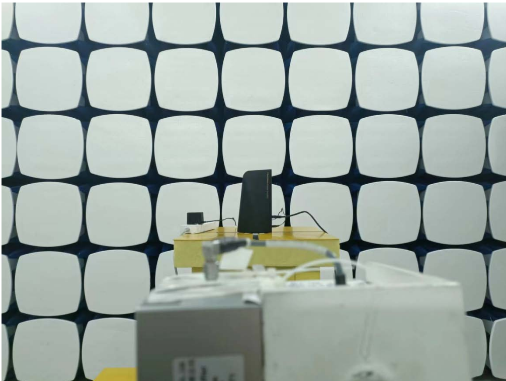
RSE (18-40) GHz
