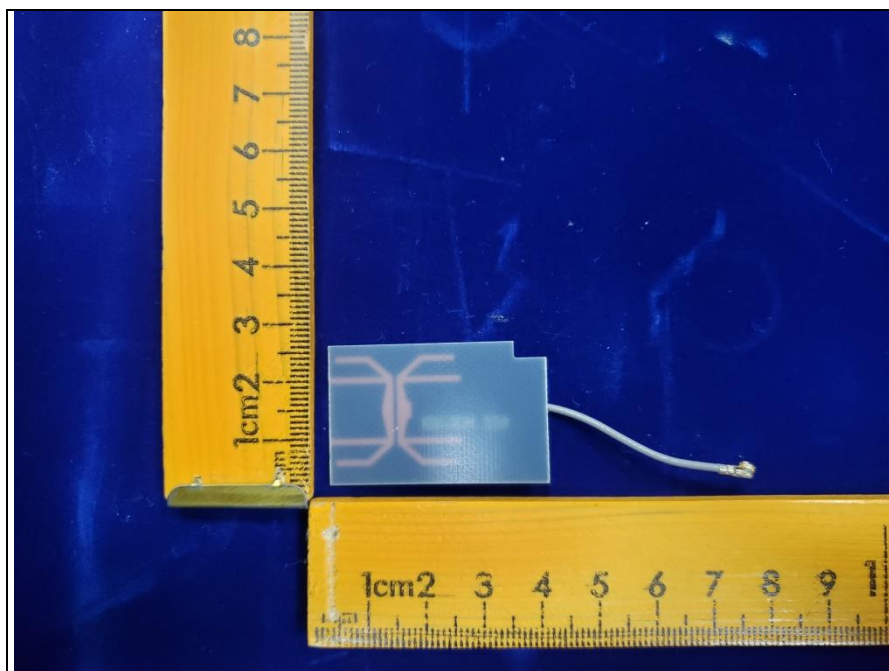
SR1021FS&SR1021F EUT-antenna (2.4G&5G WIFI Ant 3)
