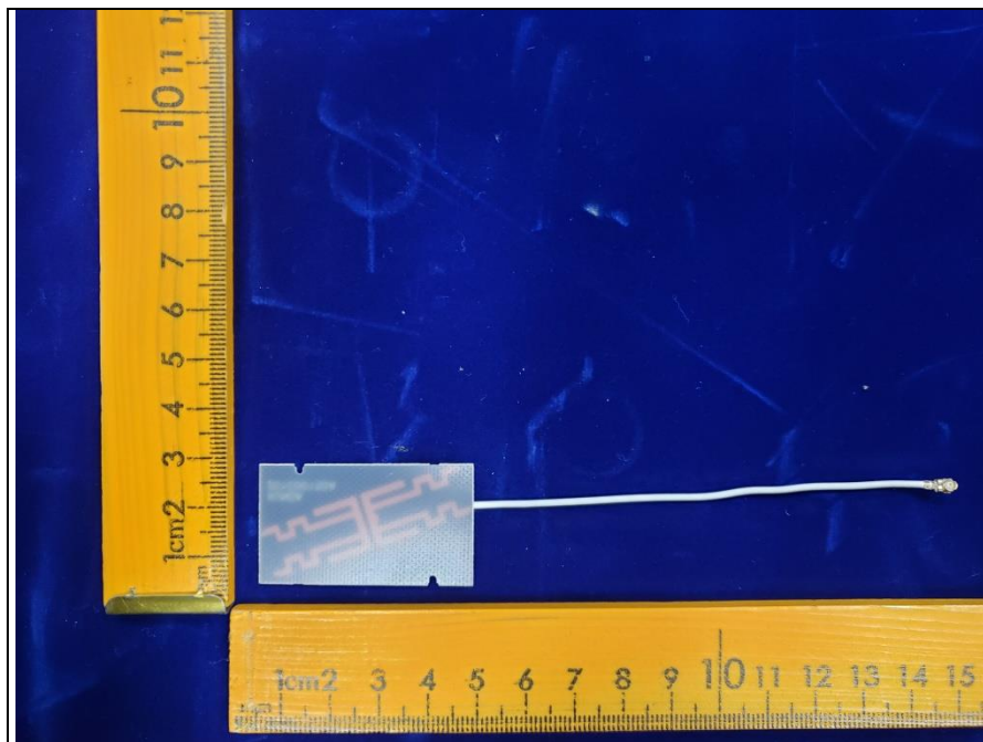
SR1021FS&SR1021F EUT-antenna (2.4G WIFI Ant 1)
