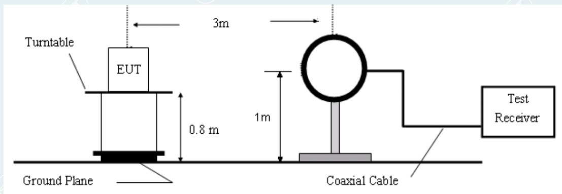
Figure 1. 1.9kHz to 30MHz radiated emissions test configuration
