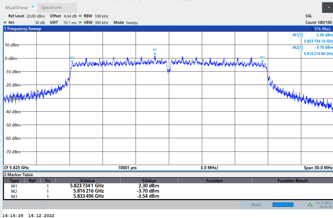
6dB Bandwidth NVNT ac20 5825MHz Ant2
