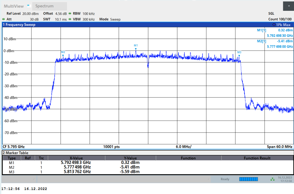
6dB Bandwidth NVNT ax40 5795MHz Ant2
