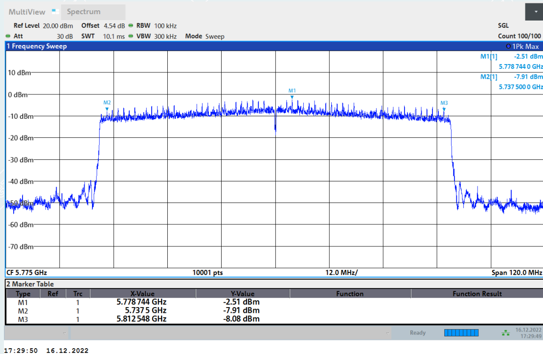
6dB Bandwidth NVNT ax80 5775MHz Ant3
