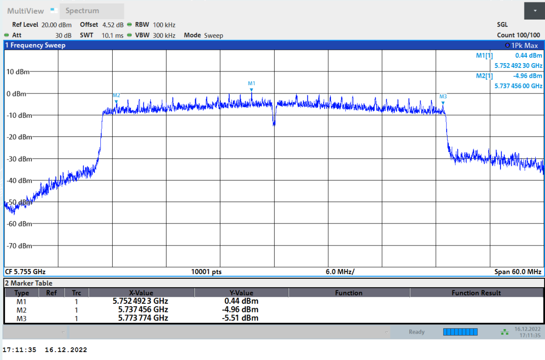
6dB Bandwidth NVNT ax40 5755MHz Ant3
