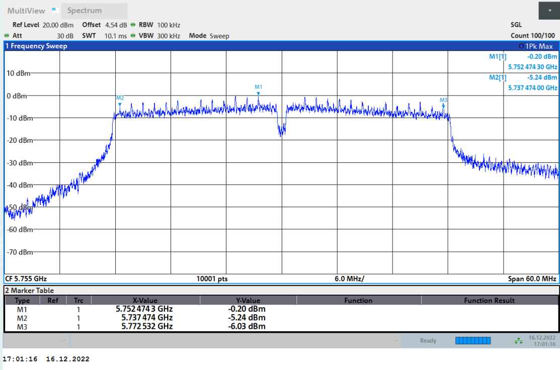
6dB Bandwidth NVNT ac40 5755MHz Ant3
