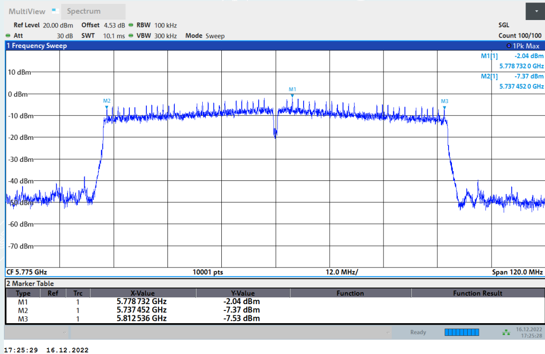
6dB Bandwidth NVNT ac80 5775MHz Ant1
