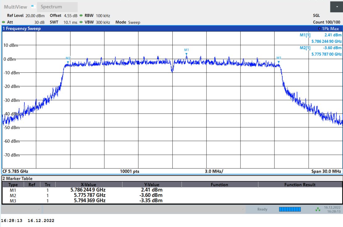
6dB Bandwidth NVNT ax20 5785MHz Ant3
