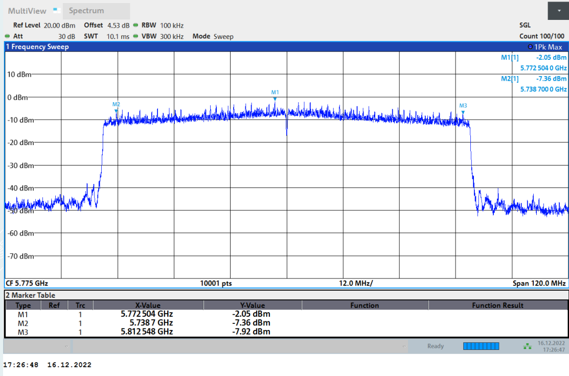
6dB Bandwidth NVNT ax80 5775MHz Ant1
