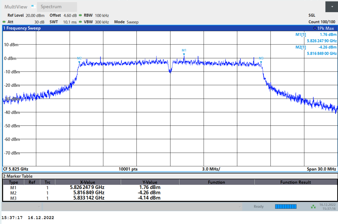
6dB Bandwidth NVNT a 5825MHz Ant2
