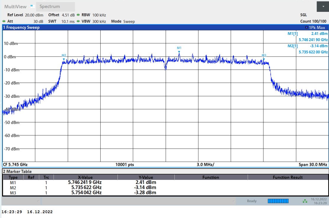
6dB Bandwidth NVNT ax20 5745MHz Ant2
