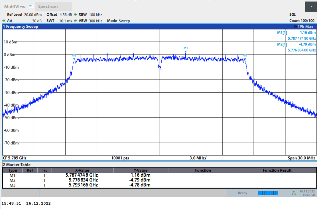
6dB Bandwidth NVNT a 5785MHz Ant3
