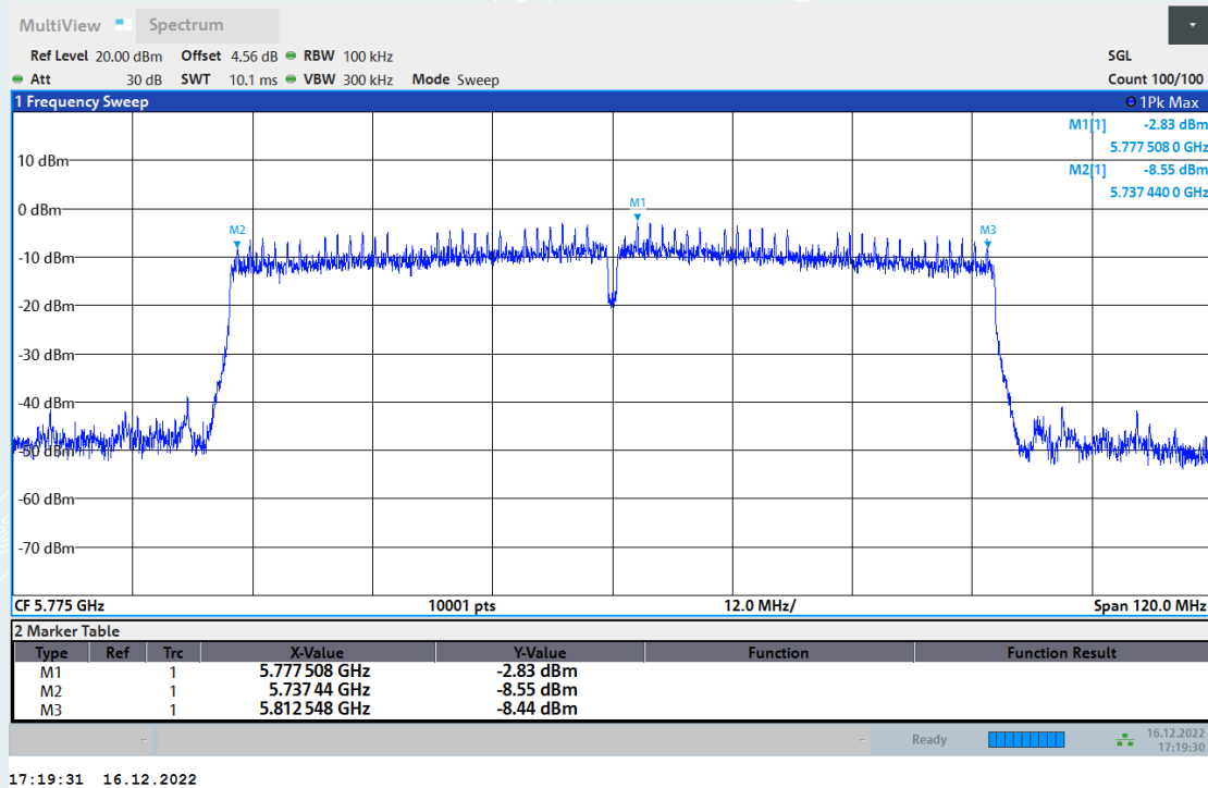
6dB Bandwidth NVNT ac80 5775MHz Ant3
