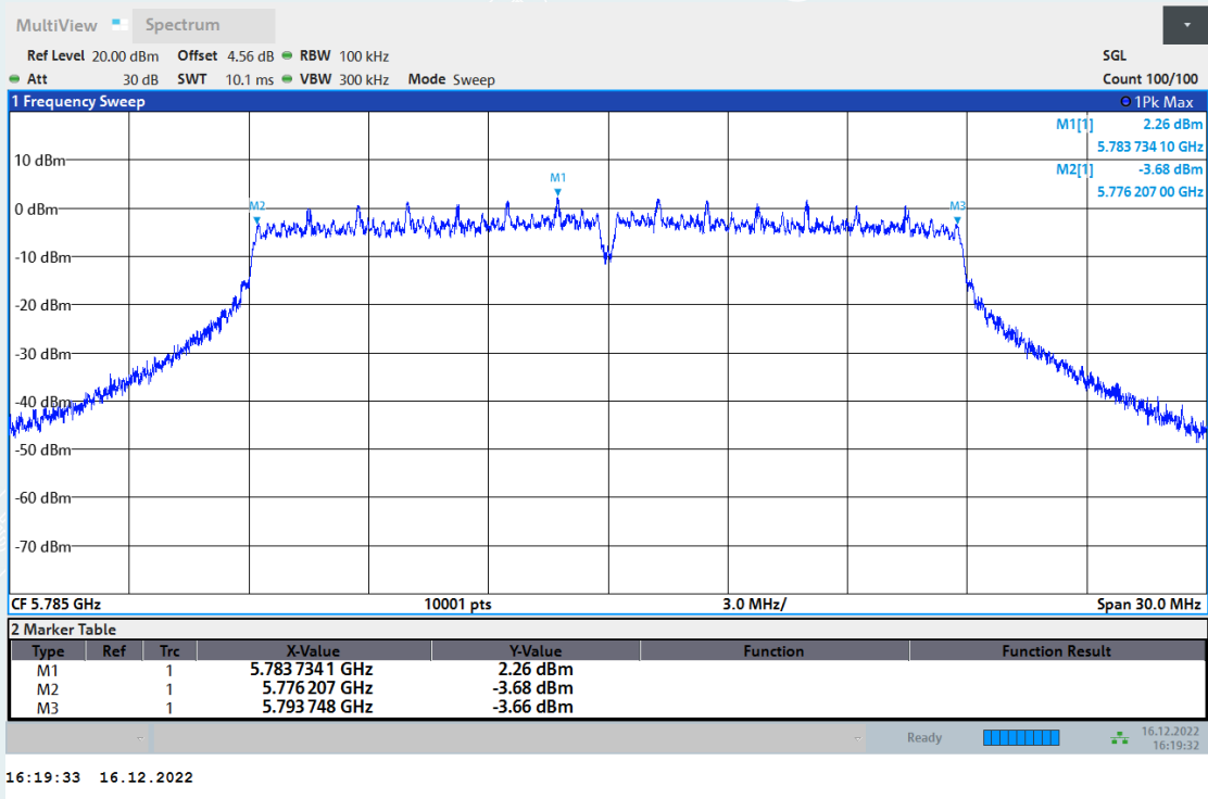
6dB Bandwidth NVNT ac20 5785MHz Ant3
