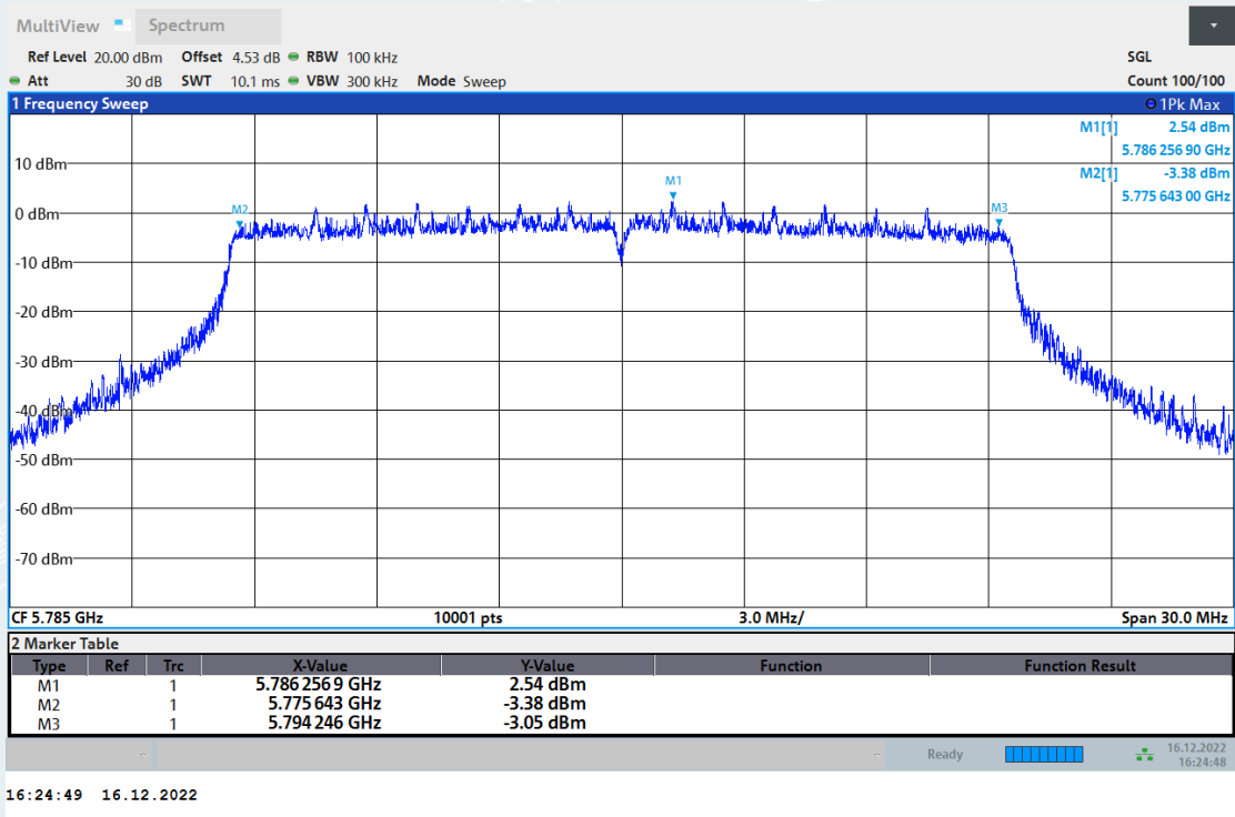
6dB Bandwidth NVNT ax20 5785MHz Ant1
