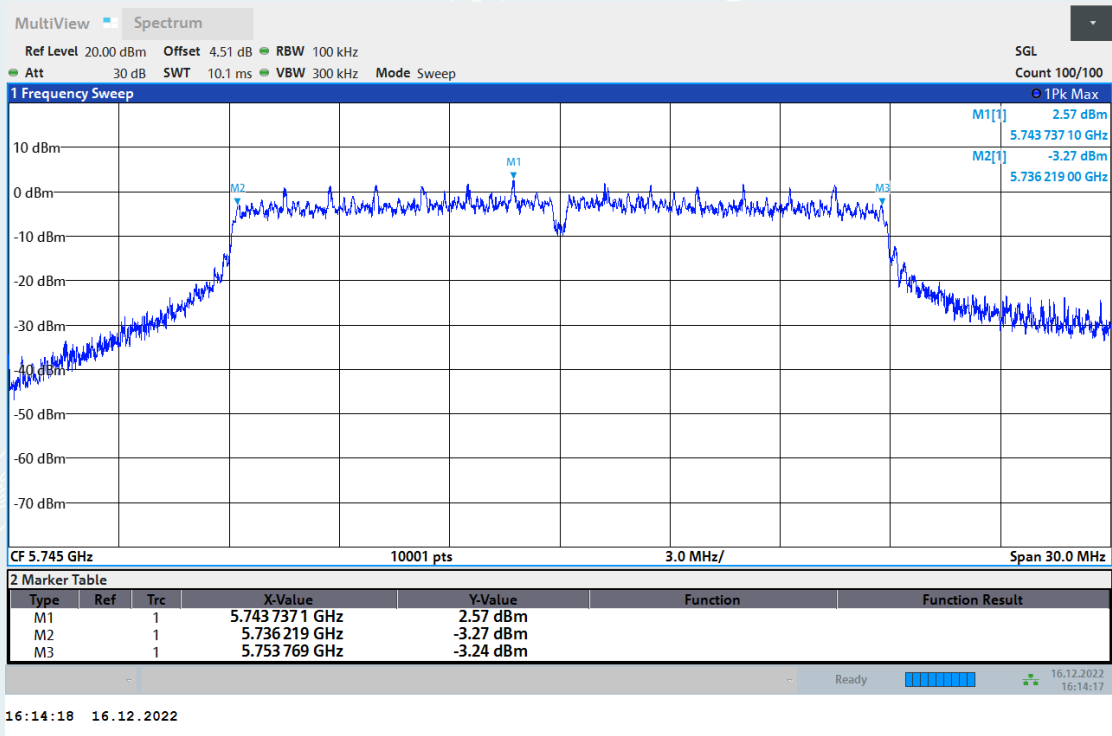
6dB Bandwidth NVNT ac20 5745MHz Ant2
