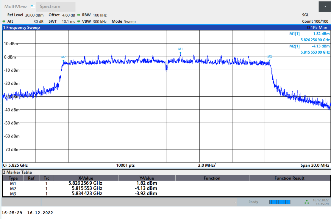
6dB Bandwidth NVNT ax20 5825MHz Ant2
