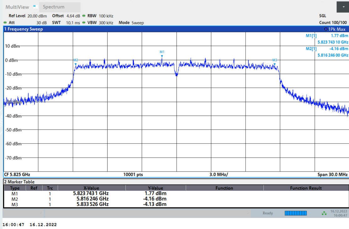
6dB Bandwidth NVNT n20 5825MHz Ant3
