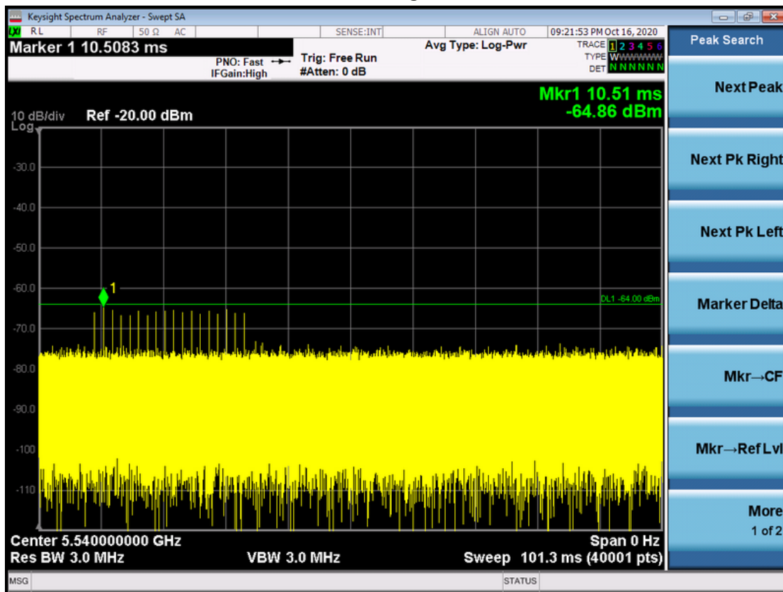
Radar Signal 0
